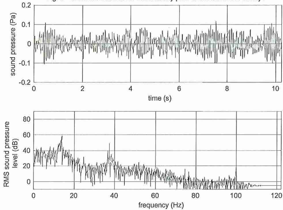
Fig. 6 - event recorded at H1 immediately prior to shutdown of Factory F
