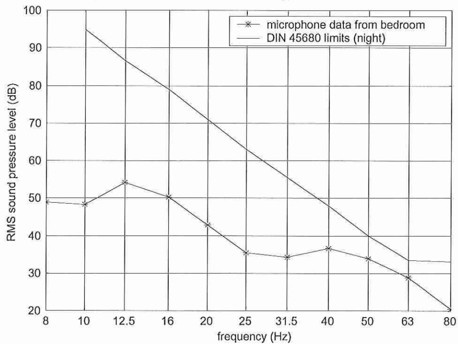
Fig. 9 - event recorded at H1 immediately after the shutdown, plotted as third-octave bands levels against DIN 45680 limits
