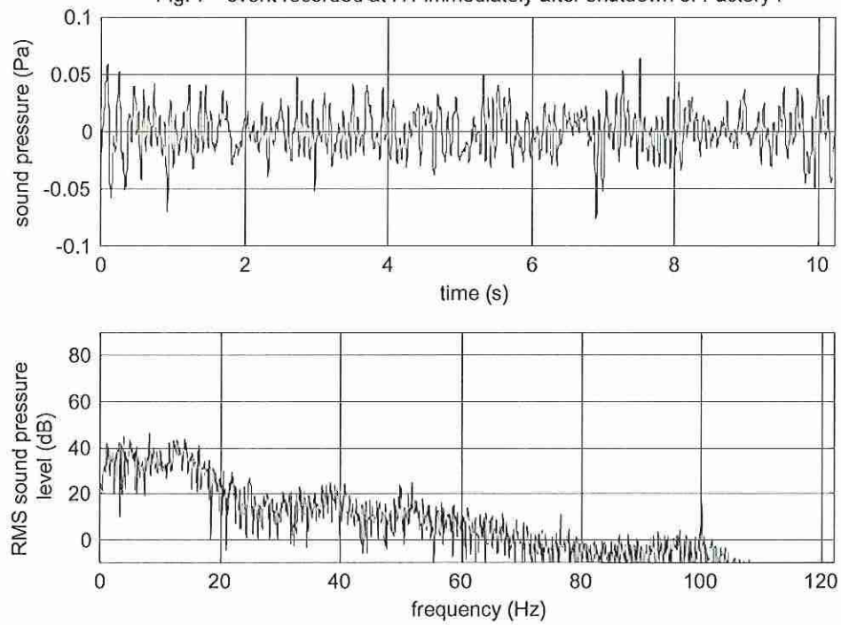
Fig. 7 - event recorded at H1 immediately after shutdown of Factory F
