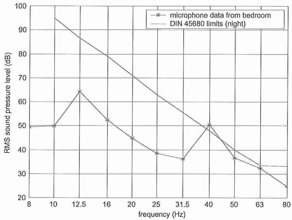
Fig. 8 - event recorded at H1 immediately prior to shutdown, plotted as third-octave bands levels against DIN 45680 limits
