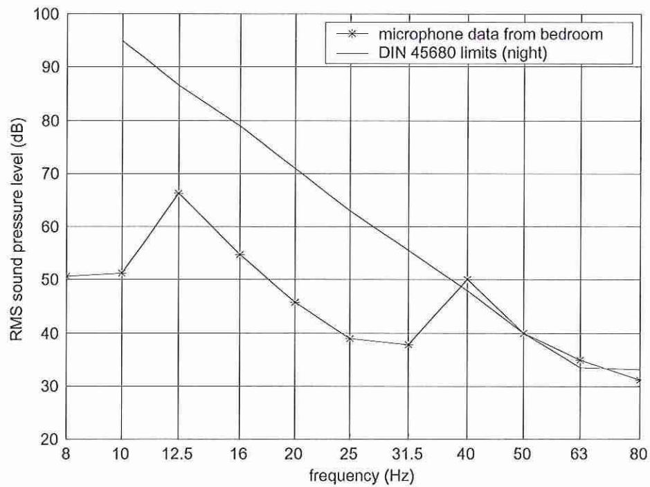
Fig. 5 - typical third-octave band levels from house H1, compared with DIN 45680 limits
