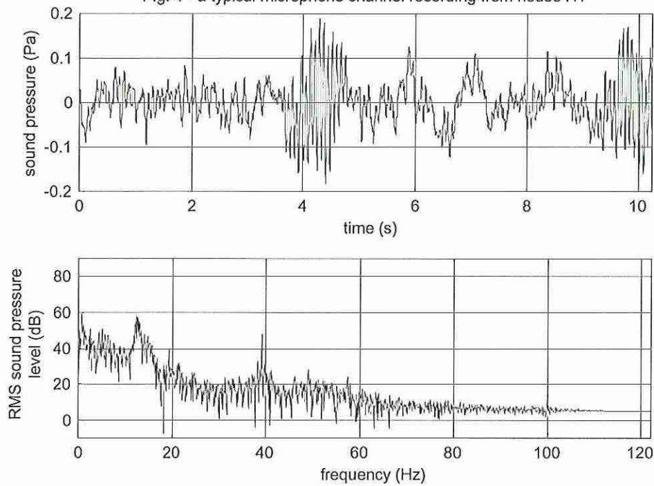
Fig. 4 - a typical microphone channel recording from house H1
