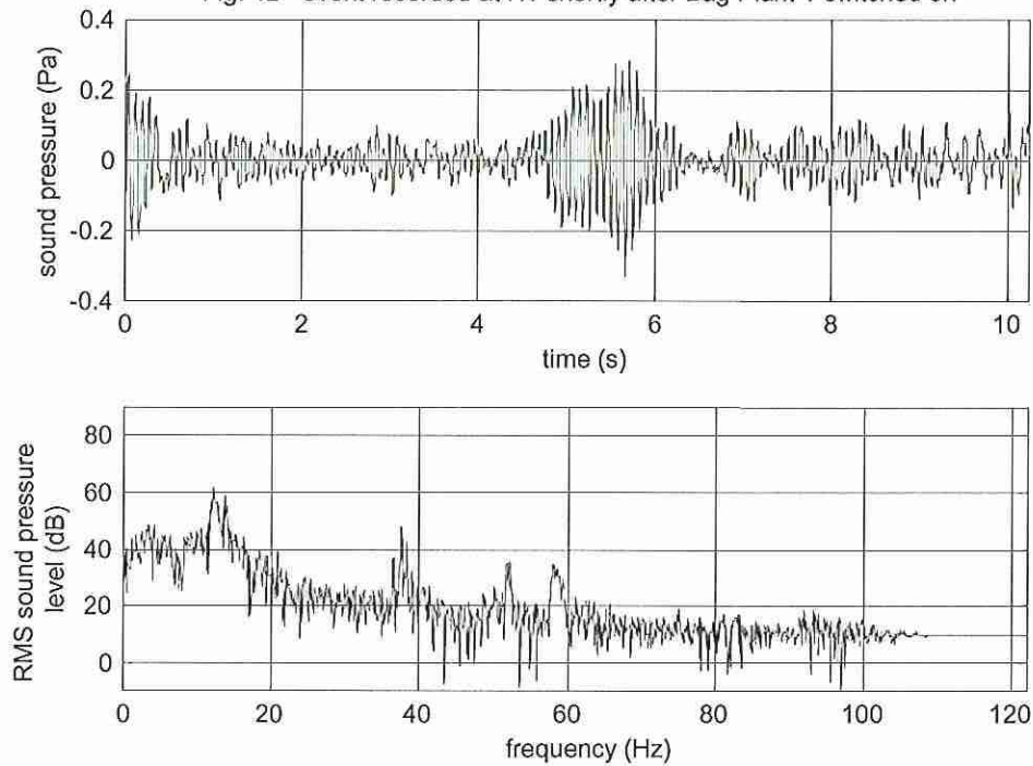
Fig. 12 - event recorded at H1 shortly after Bag Plant 1 switched on
