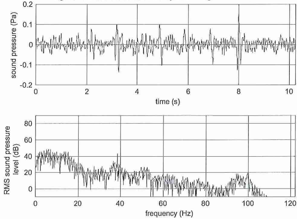
Fig. 10 - event recorded at H1 shortly before Bag Plant 2 switched on
