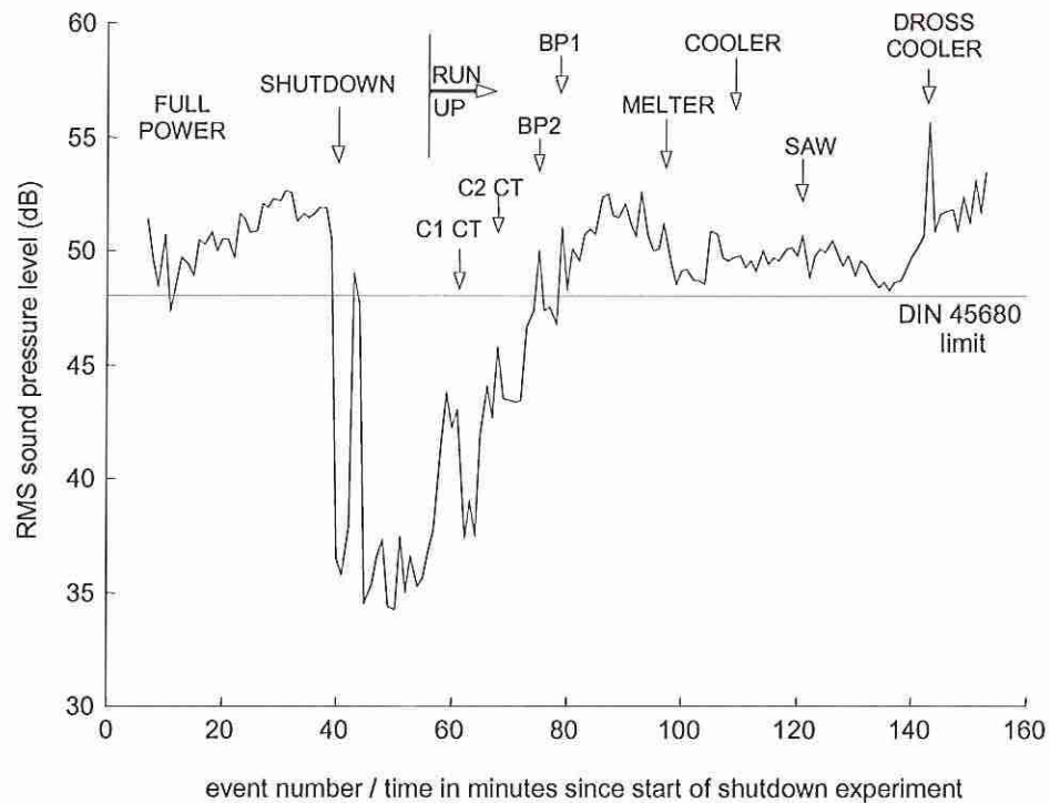
Fig. 13 - variations in 40 Hz third-octave band level throughout the shutdown experiment, with details of plant activity (C1 CT = Caster 1 Cooling Tower; C2 CT = Caster 2 Cooling Tower; BP1 = Bag Plant 1; BP2 = Bag Plant 2)
