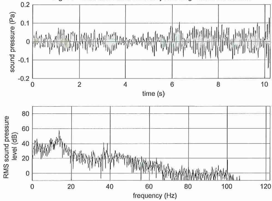
Fig. 11 - event recorded at H1 shortly after Bag Plant 2 switched on
