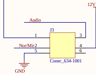
Camera connector
