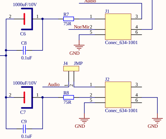
DVR connector
