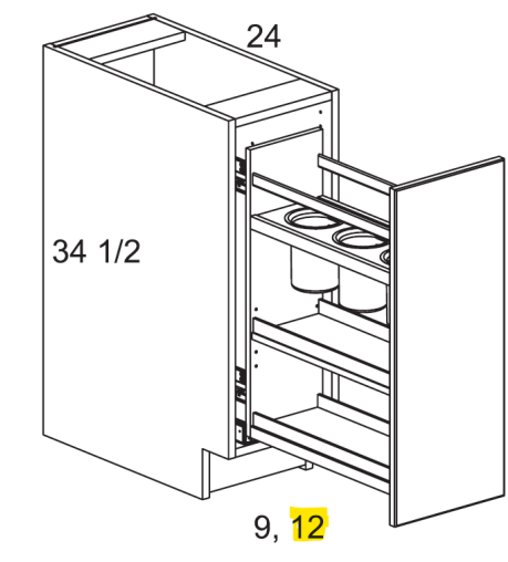
SPICE PULLOUTS - SSP02/3/4/6 40/50/60/70
