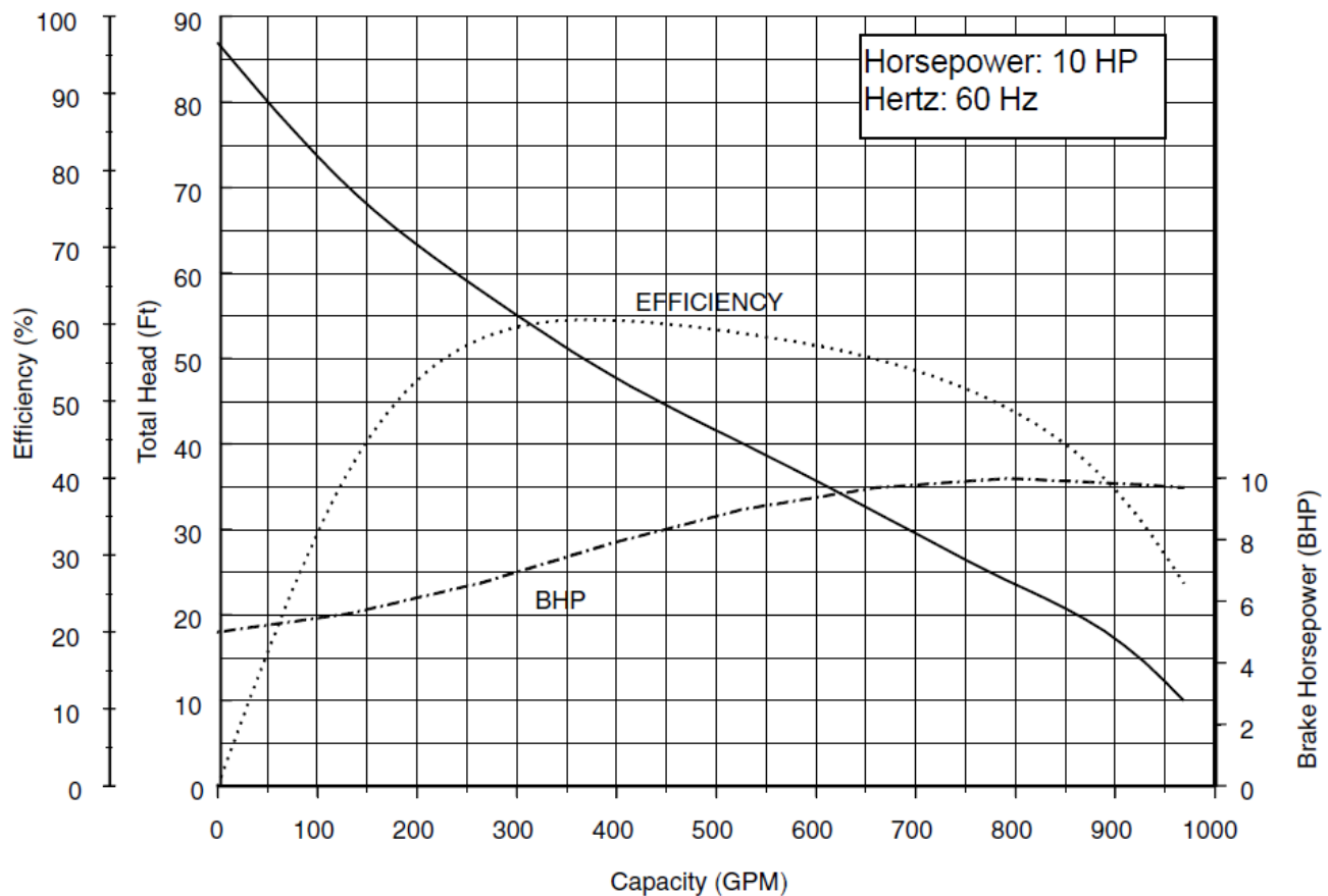
Stancor Model 100LX67.5 Individual Performance Curve
