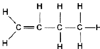
hydrocarbon 2
