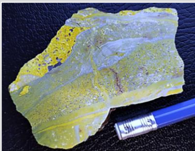
AMSEL TARGET, BIG TEN, NEVADA banded quartz-adularia with py in tuffisite
