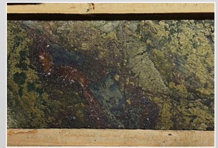
HECLA-KILMER PROJECT, ONTARIO iron oxide - copper-gold breccia
