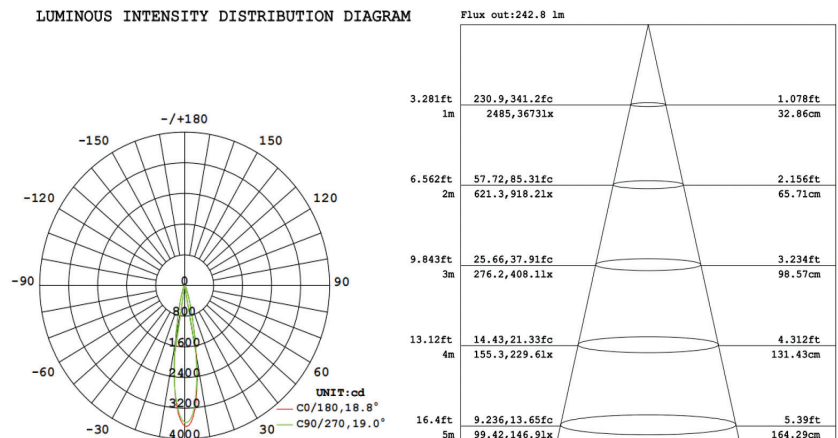
LUMINOUS INTENSITY DISTRIBUTION DIAGRAM
