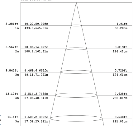
Flux out: 127.1 lm
