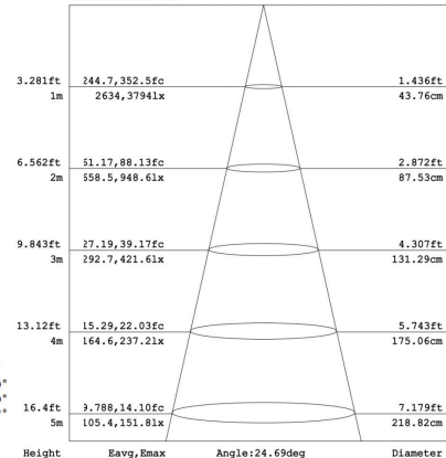
Flux out: 441.0 lm
