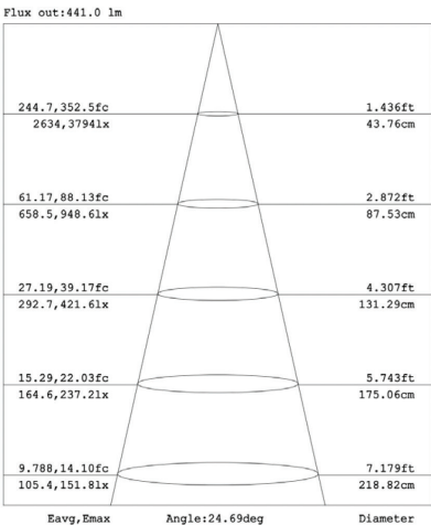
LUMINOUS INTENSITY DISTRIBUTION DIAGRAM
