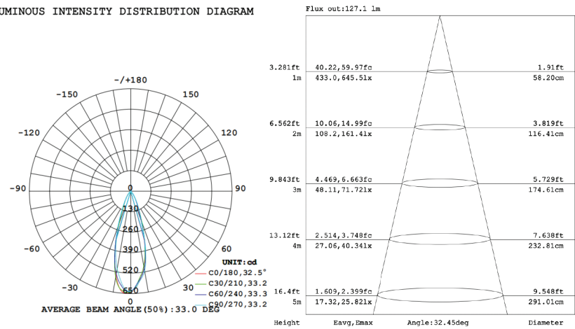
LUMINOUS INTENSITY DISTRIBUTION DIAGRAM
