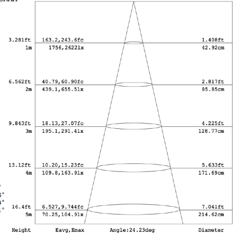
Flux out: 294.1 lm
