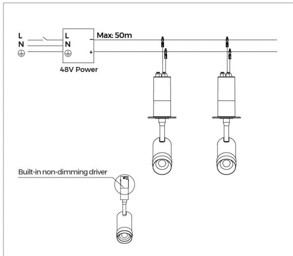
ON/OFF wiring diagram
