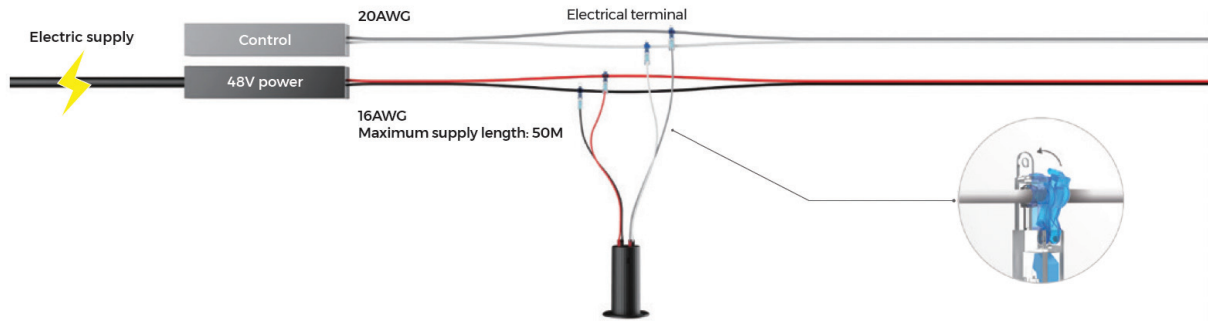
ON/OFF wiring diagram
