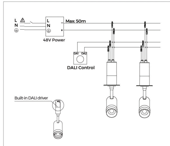
DALI wiring diagram
