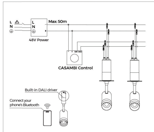
CASAMBI wiring diagram
