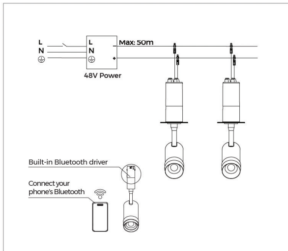
Tuya Bluetooth wiring diagram
