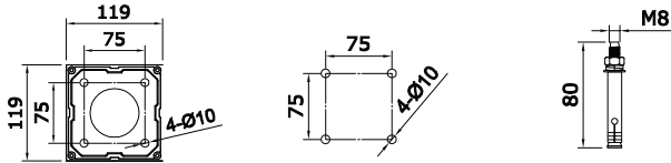
Installation Hole Size
