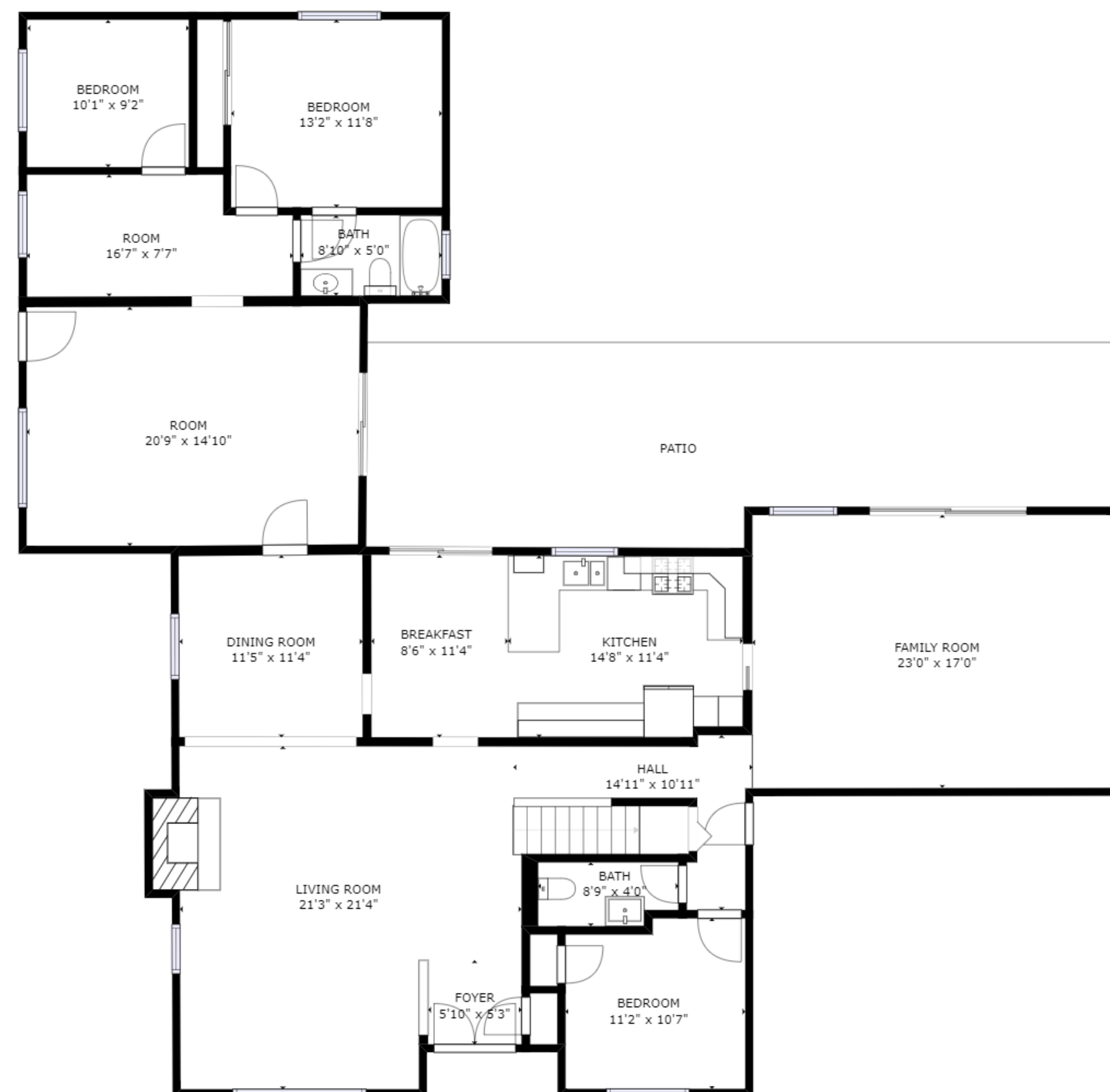
FLOOR 1
