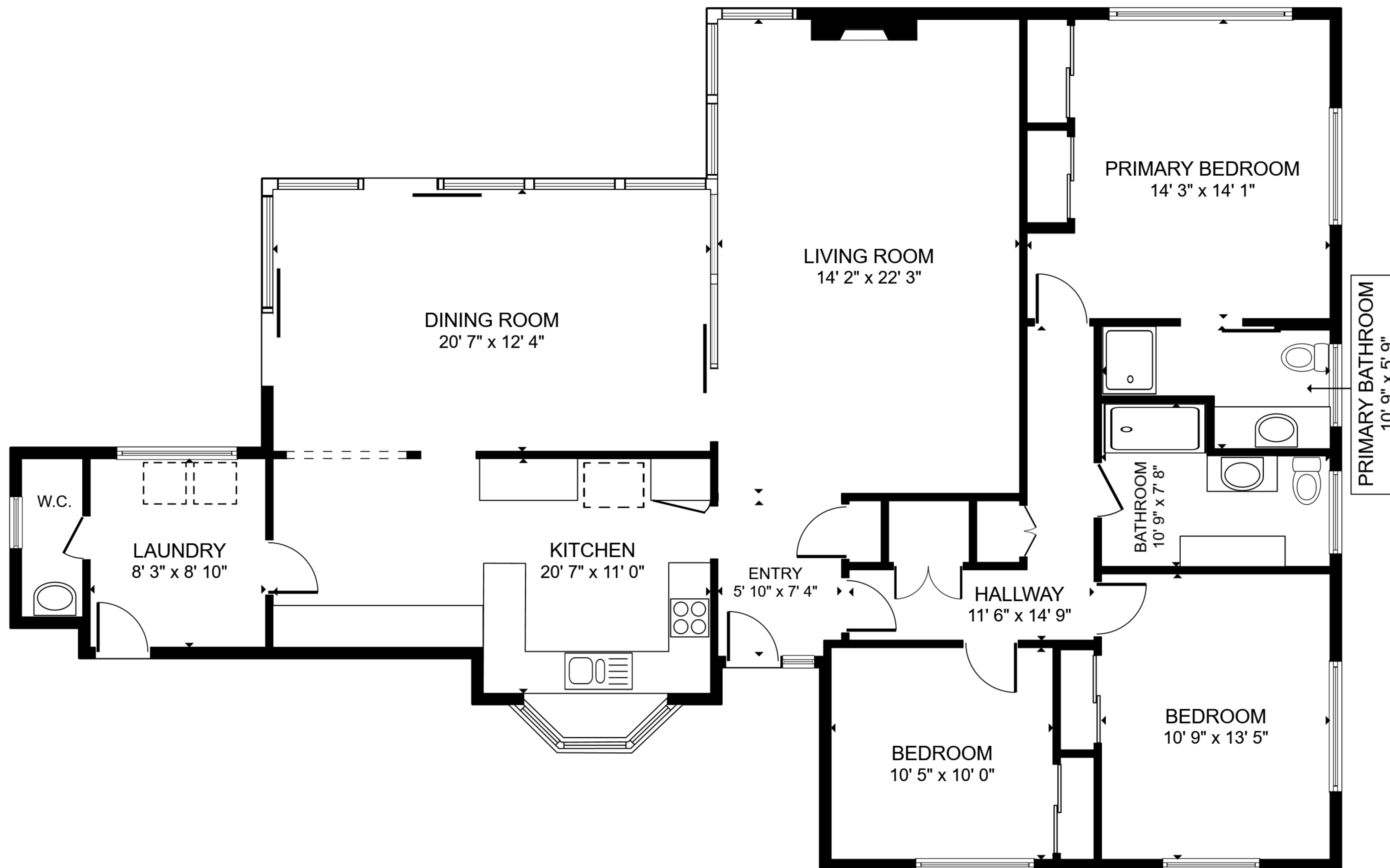
FLOOR PLAN
