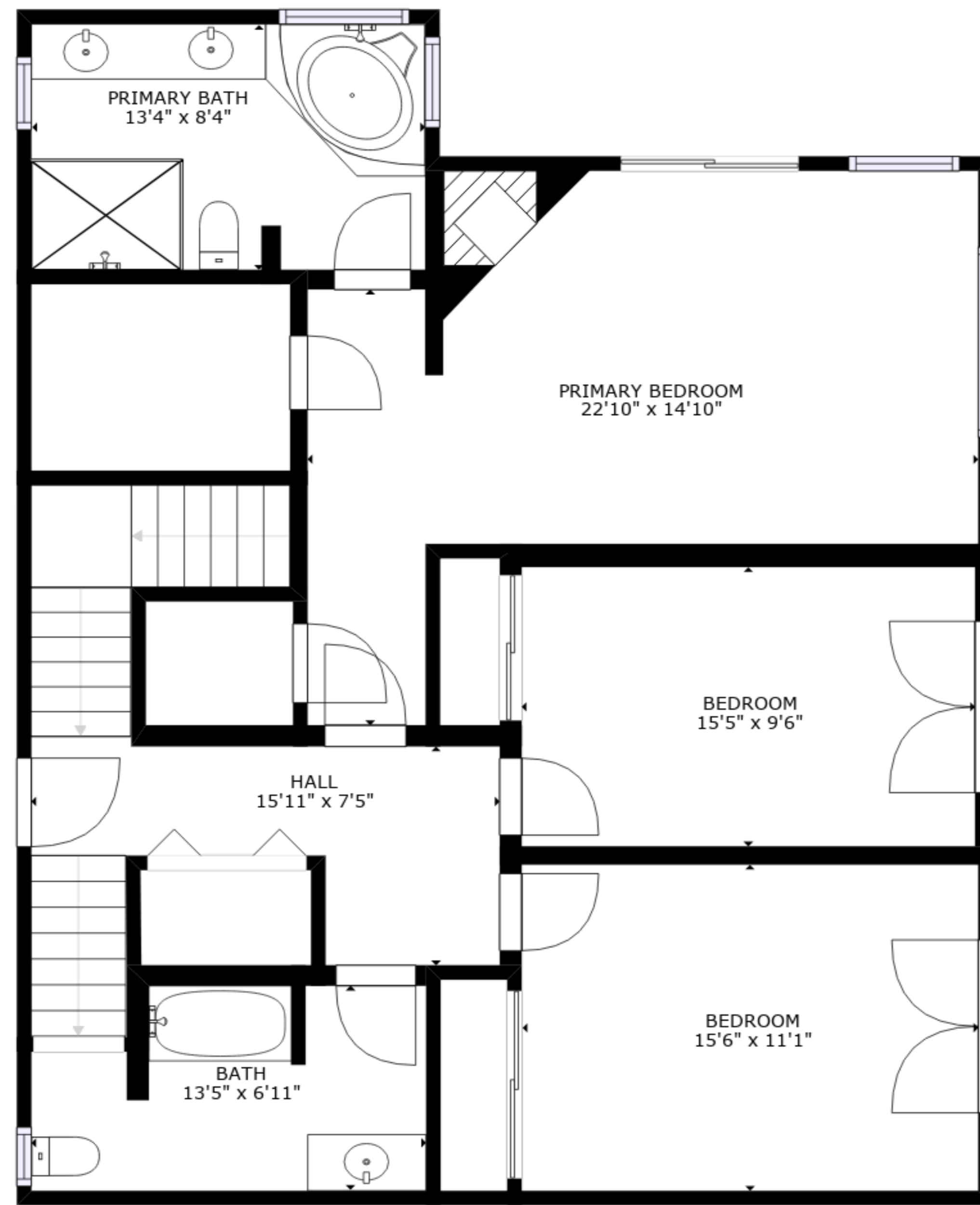
FLOOR 2
