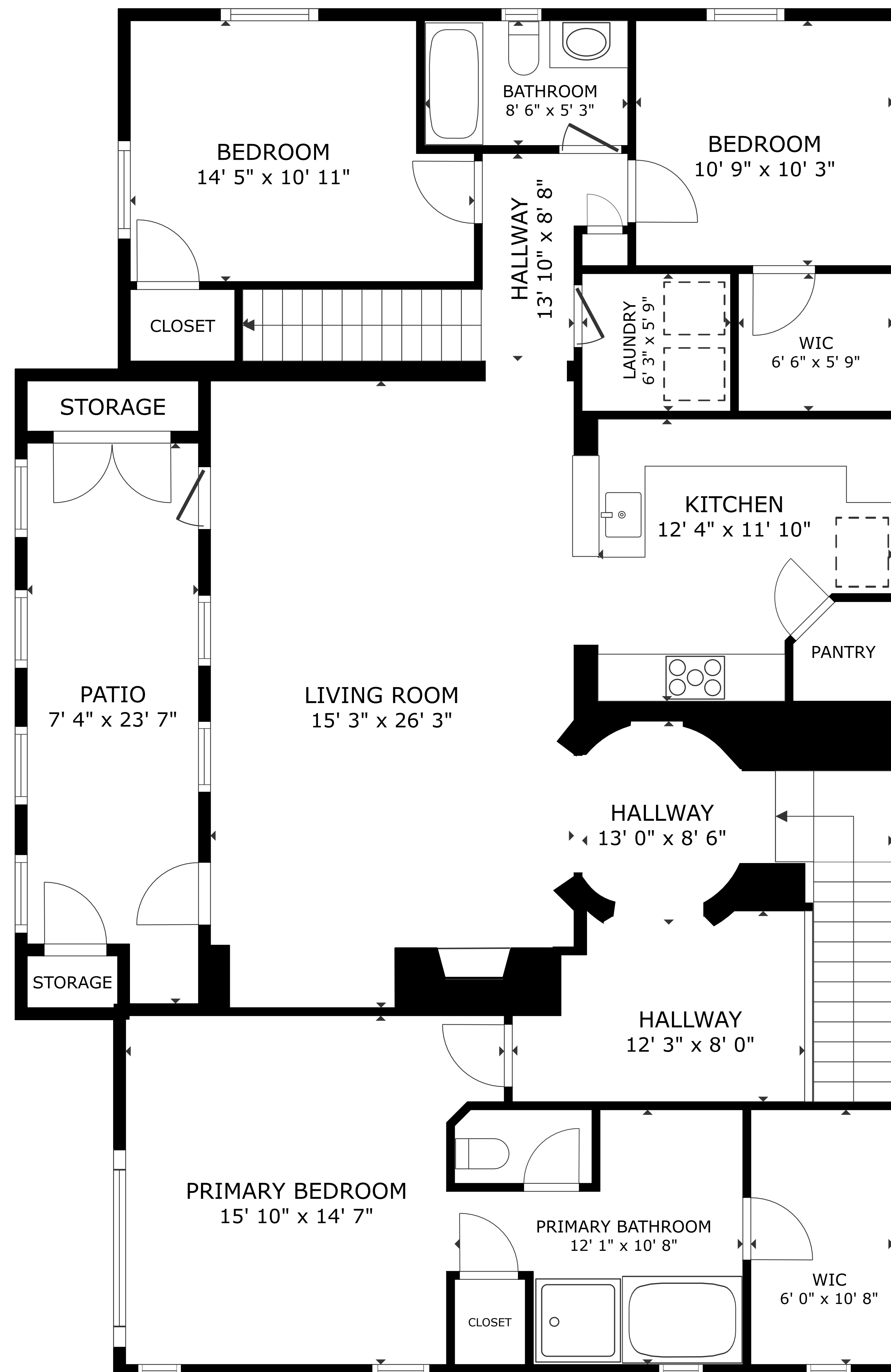
FLOOR 2
