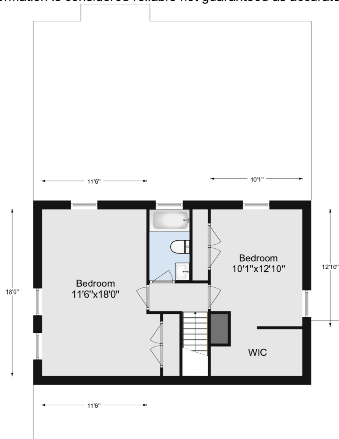
2nd Floor
