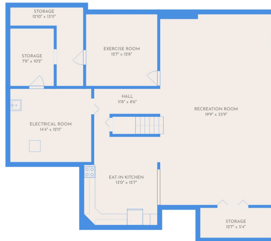
FLOOR 1
