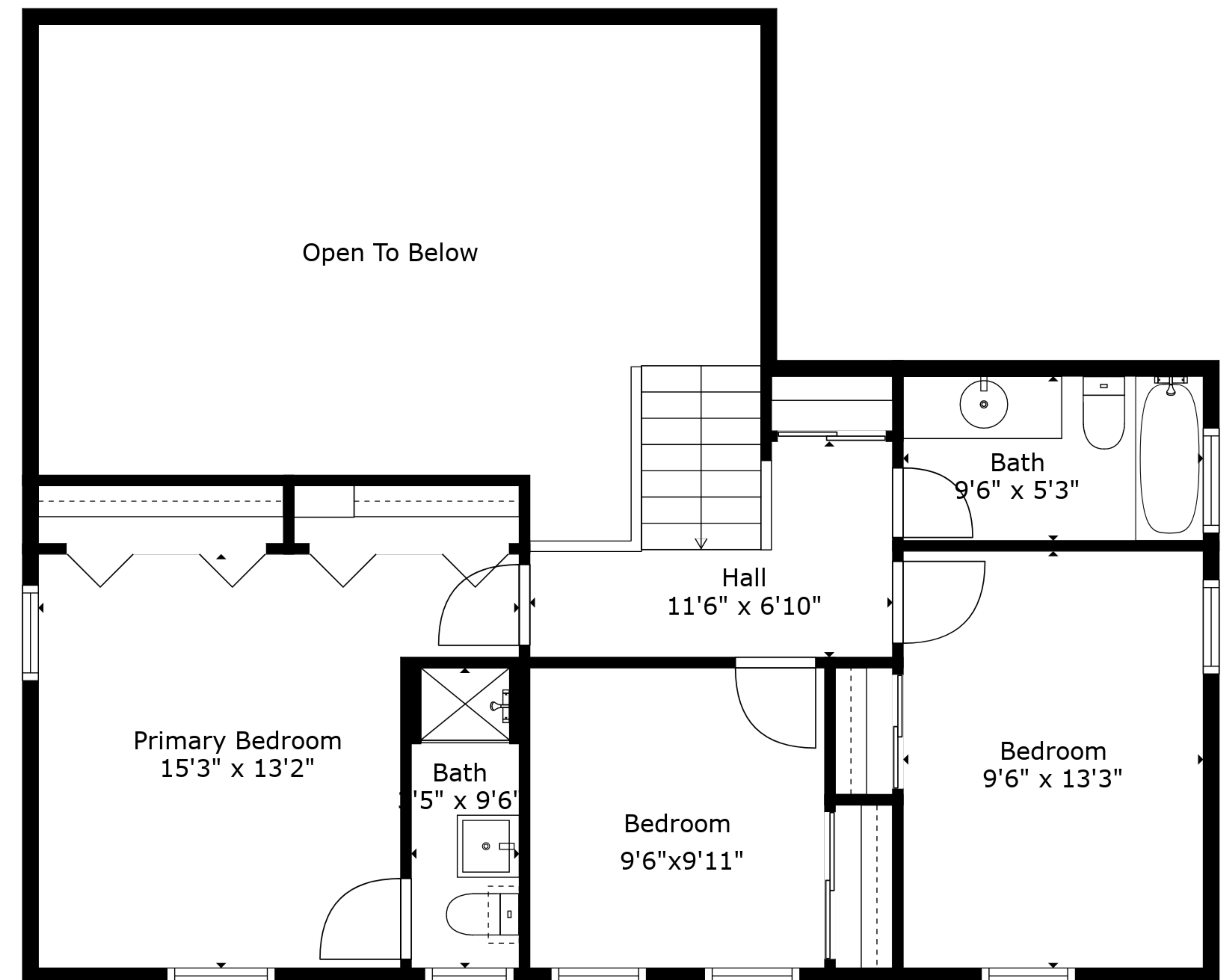
Floor 3
