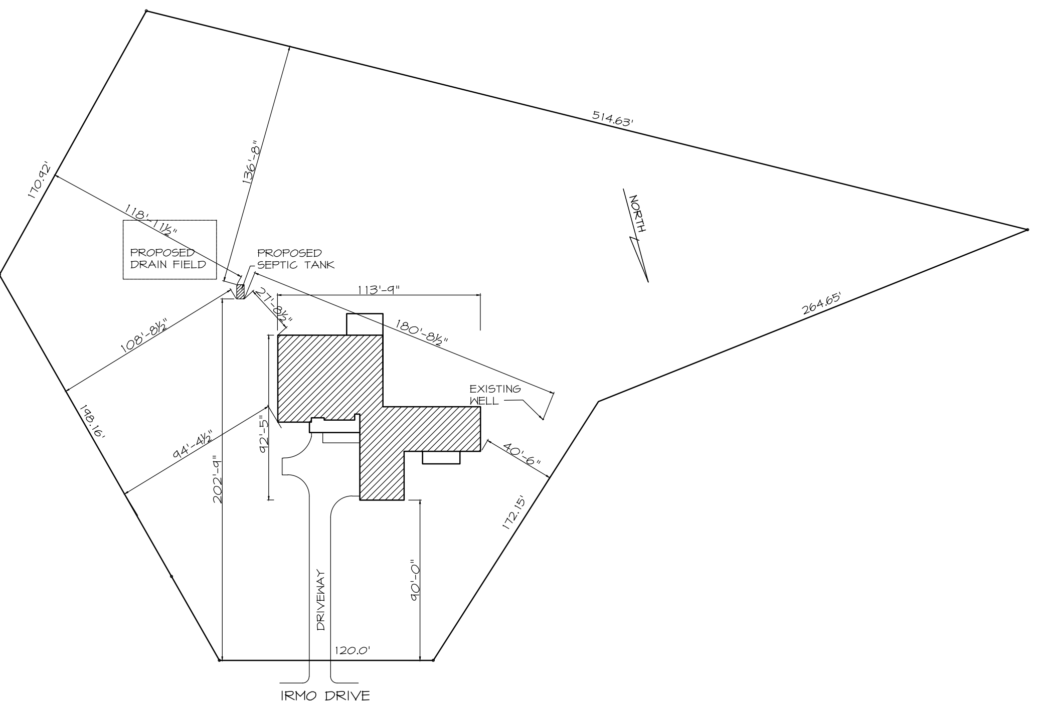
PLOT PLAN
