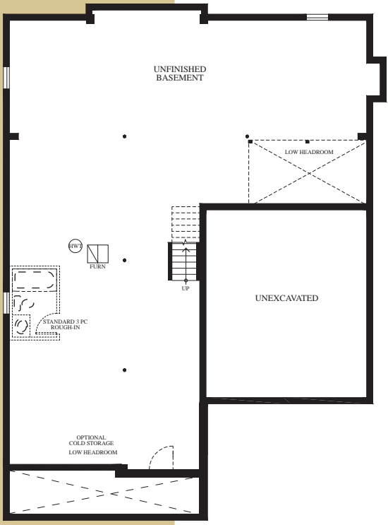
Basement Elevation 'D'
