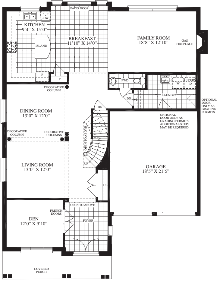
Ground Floor Elevation 'D'
