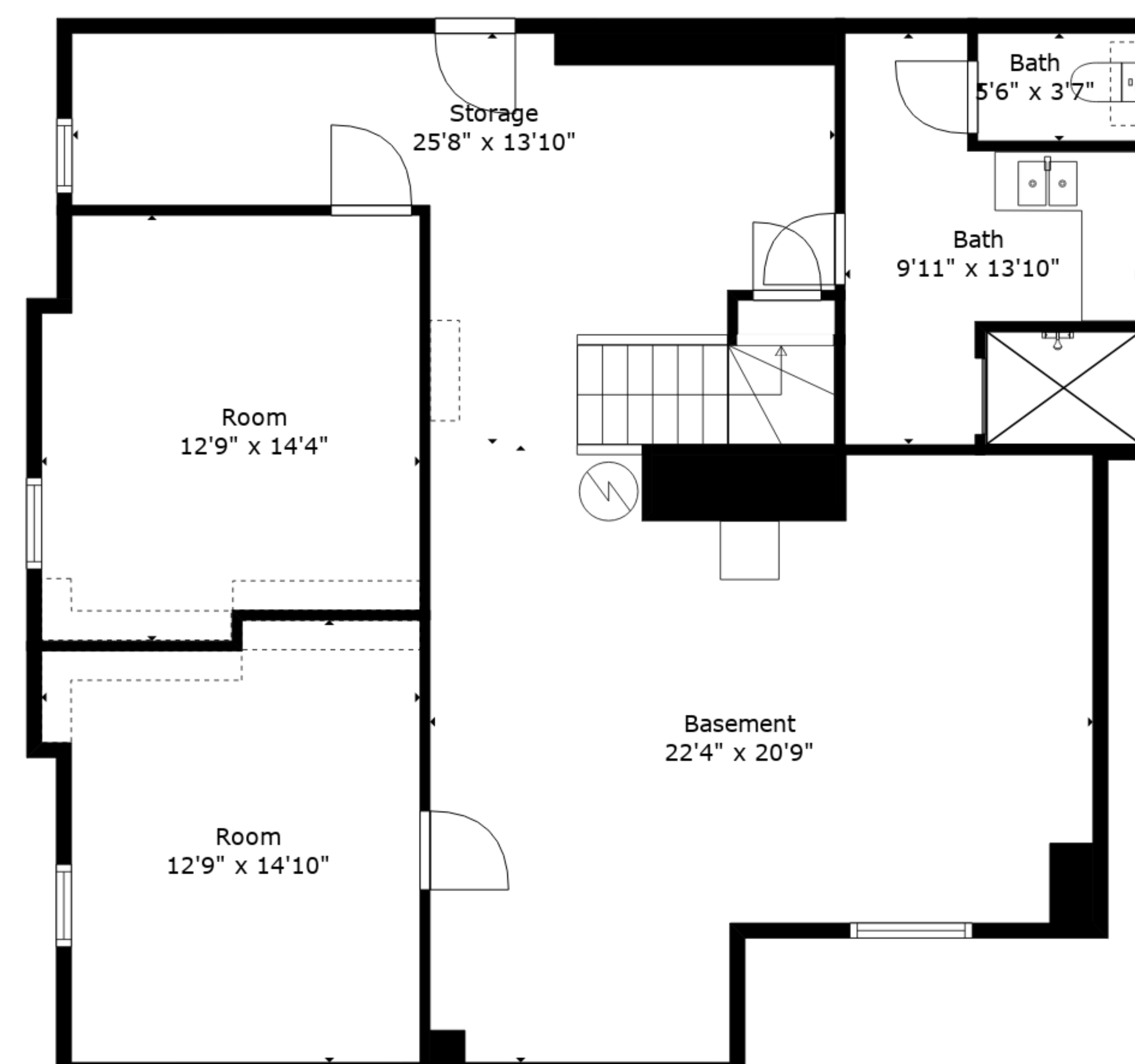
Floor 1
