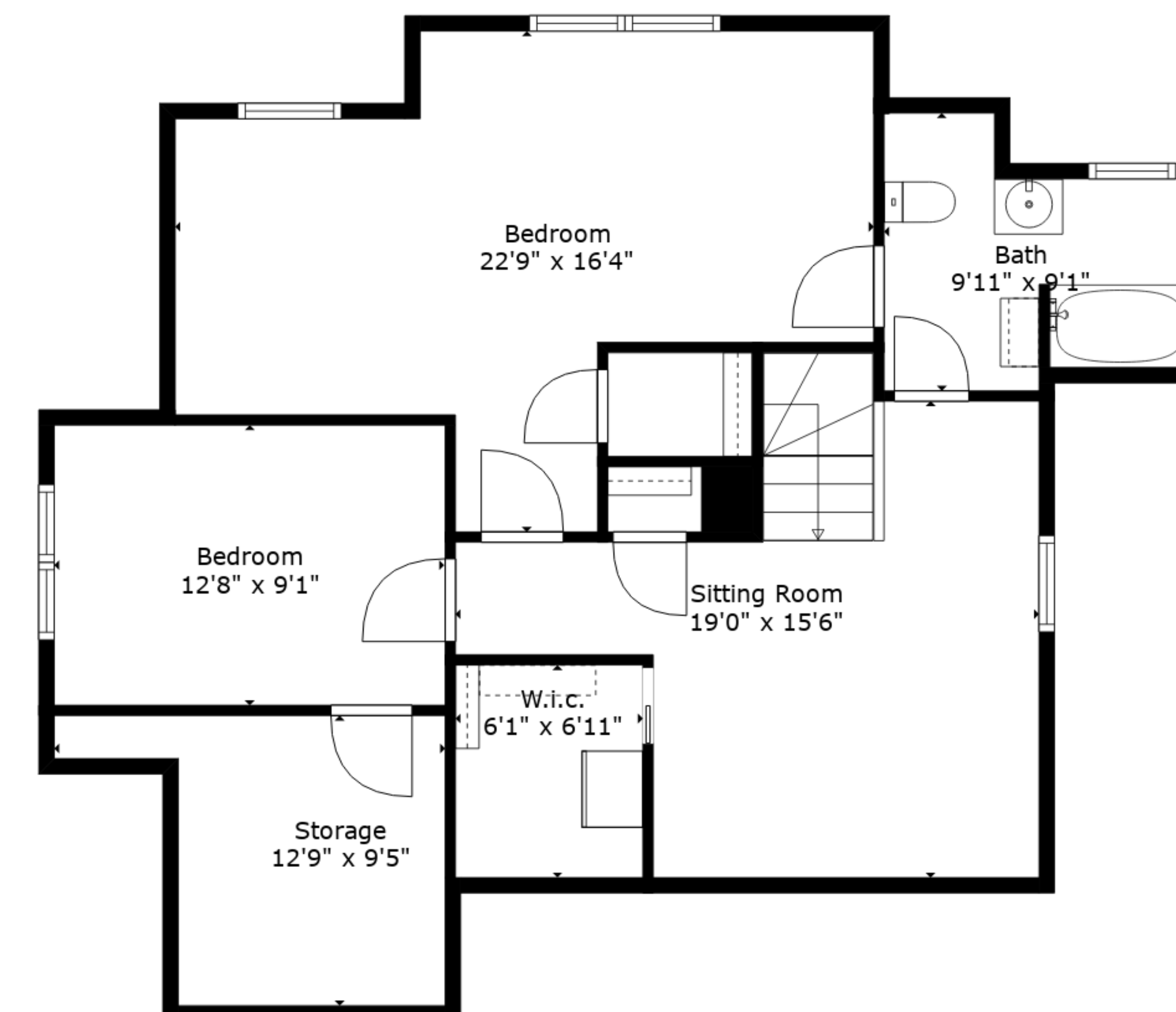
Floor 3
