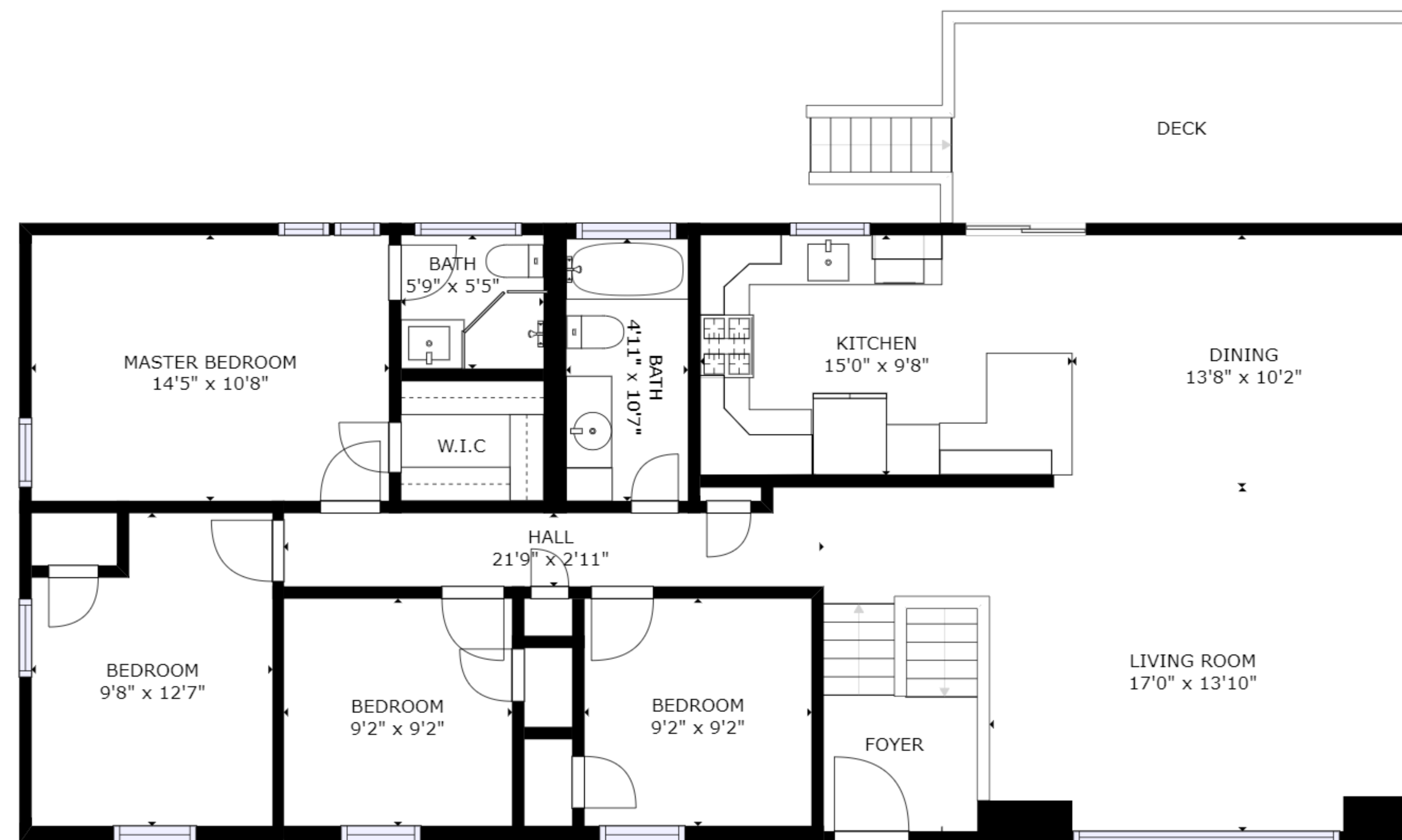
FLOOR 2
