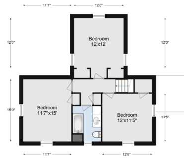
Cottage Level 2 Floor plans are intended to give a general indication of the layout. The information is considered reliable not guaranteed as accurate or complete.
