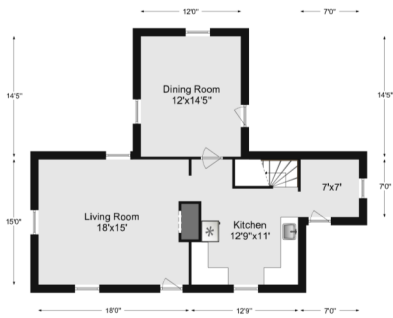
Cottage Level 1 Floor plans are intended to give a general indication of the layout. The information is considered reliable not guaranteed as accurate or complete.
