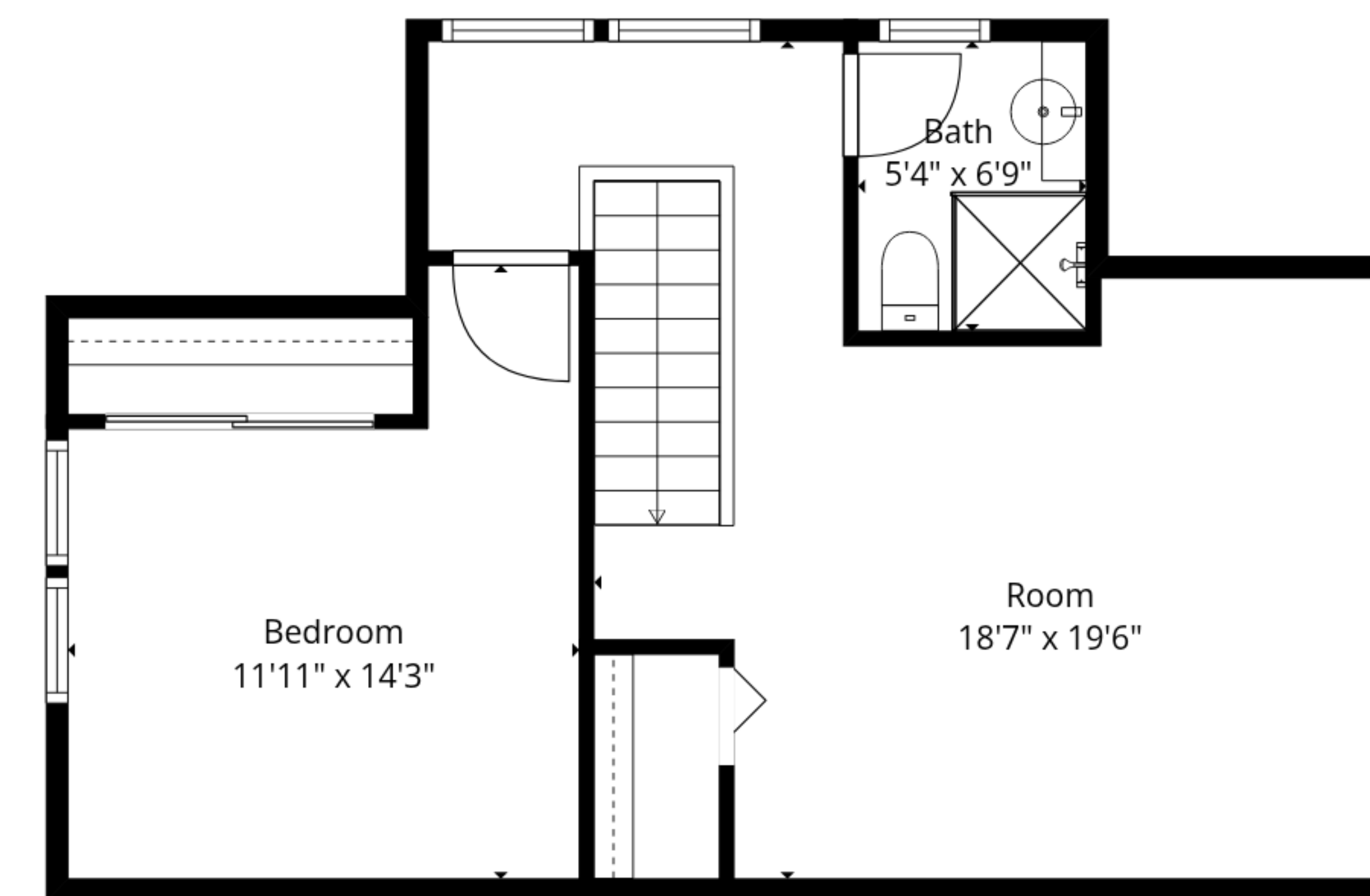
Floor 3
