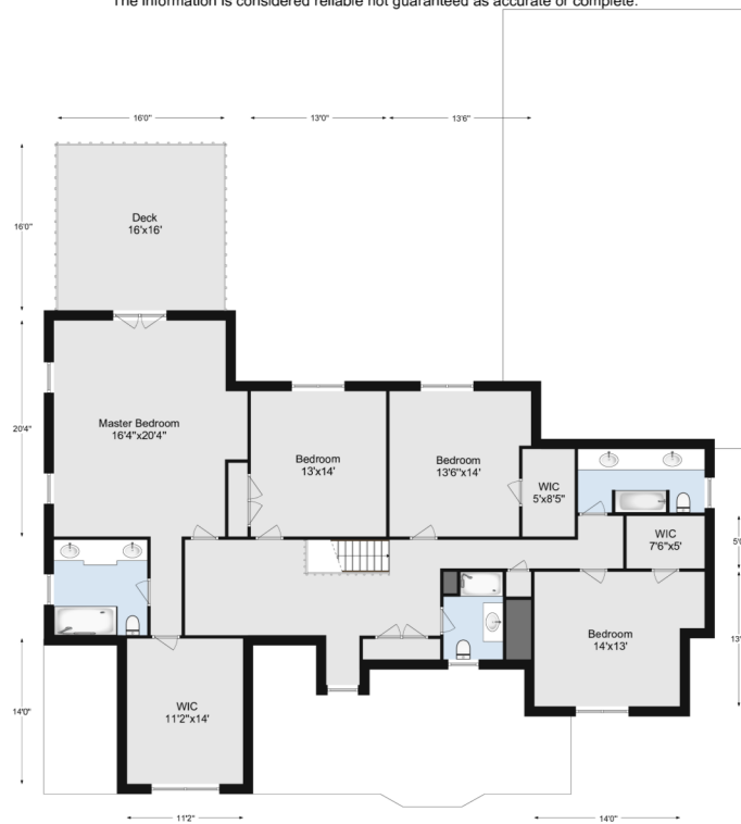
2nd Floor
