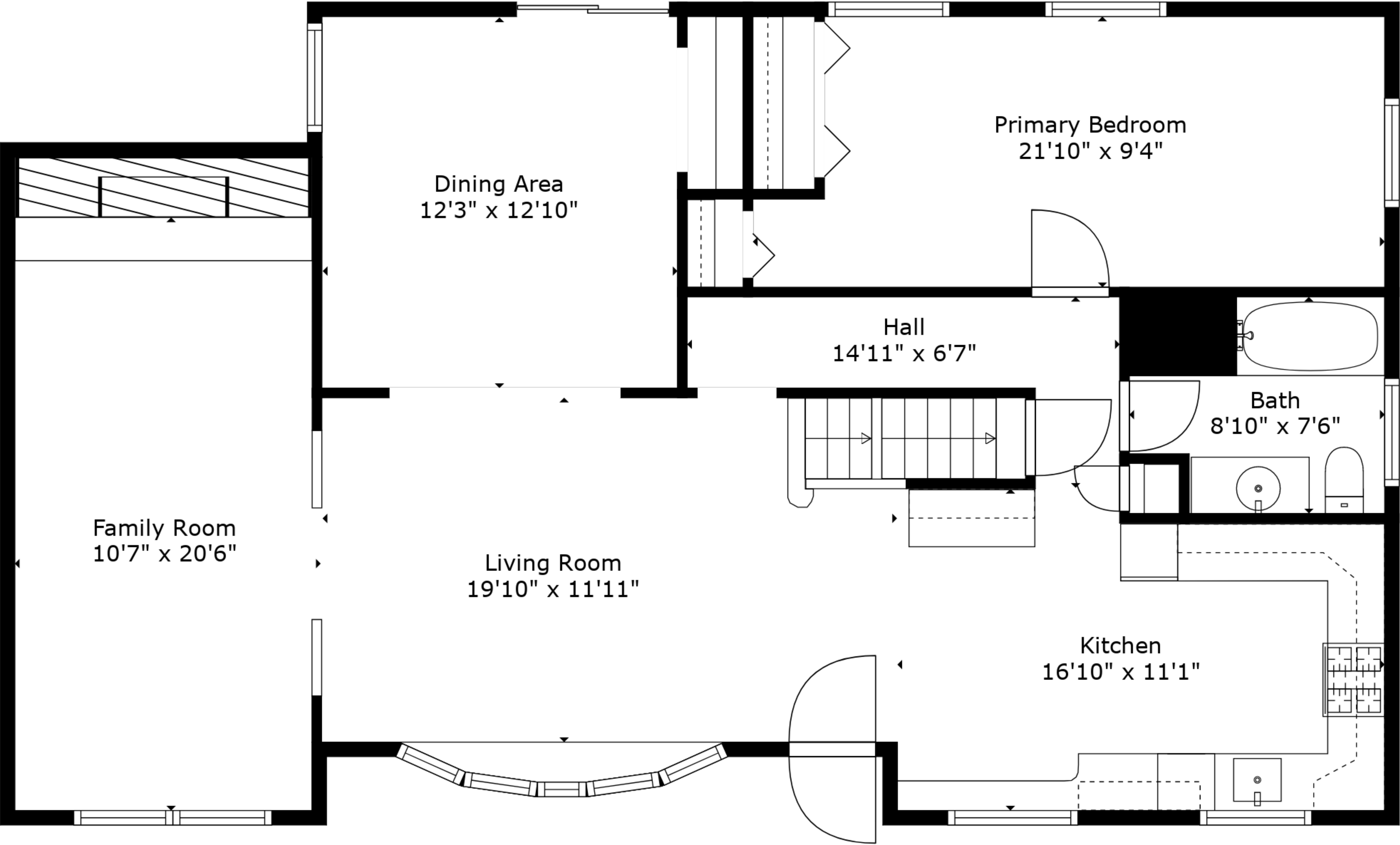
Floor 2
