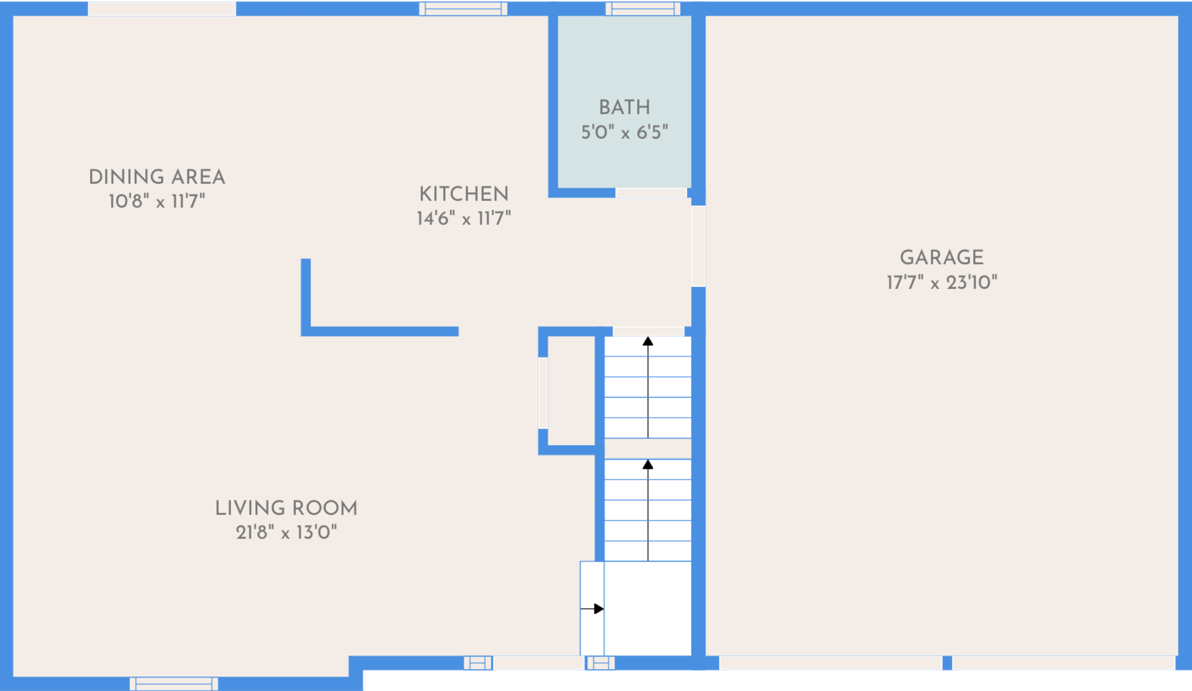
FLOOR 2
