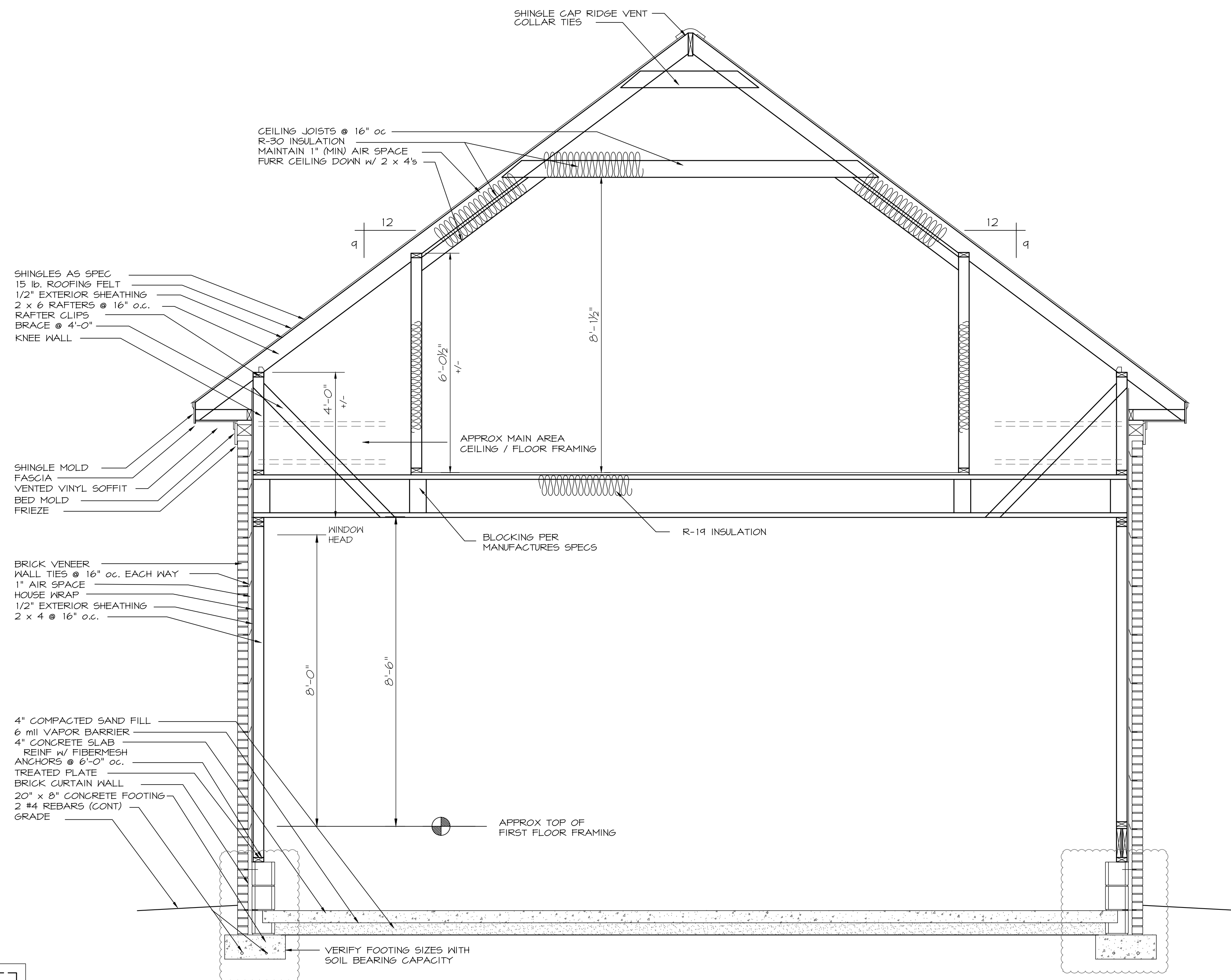
GARAGE SECTION
