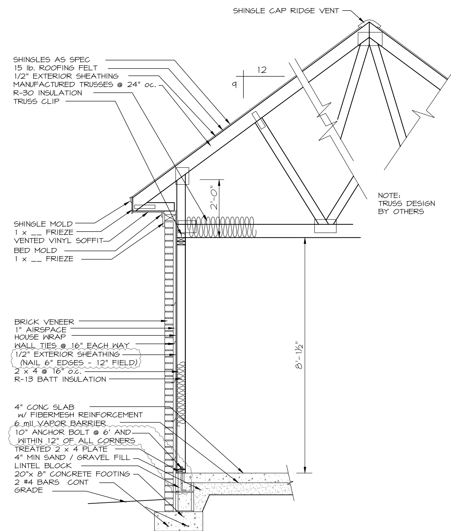
APARTMENT WALL SECTION
