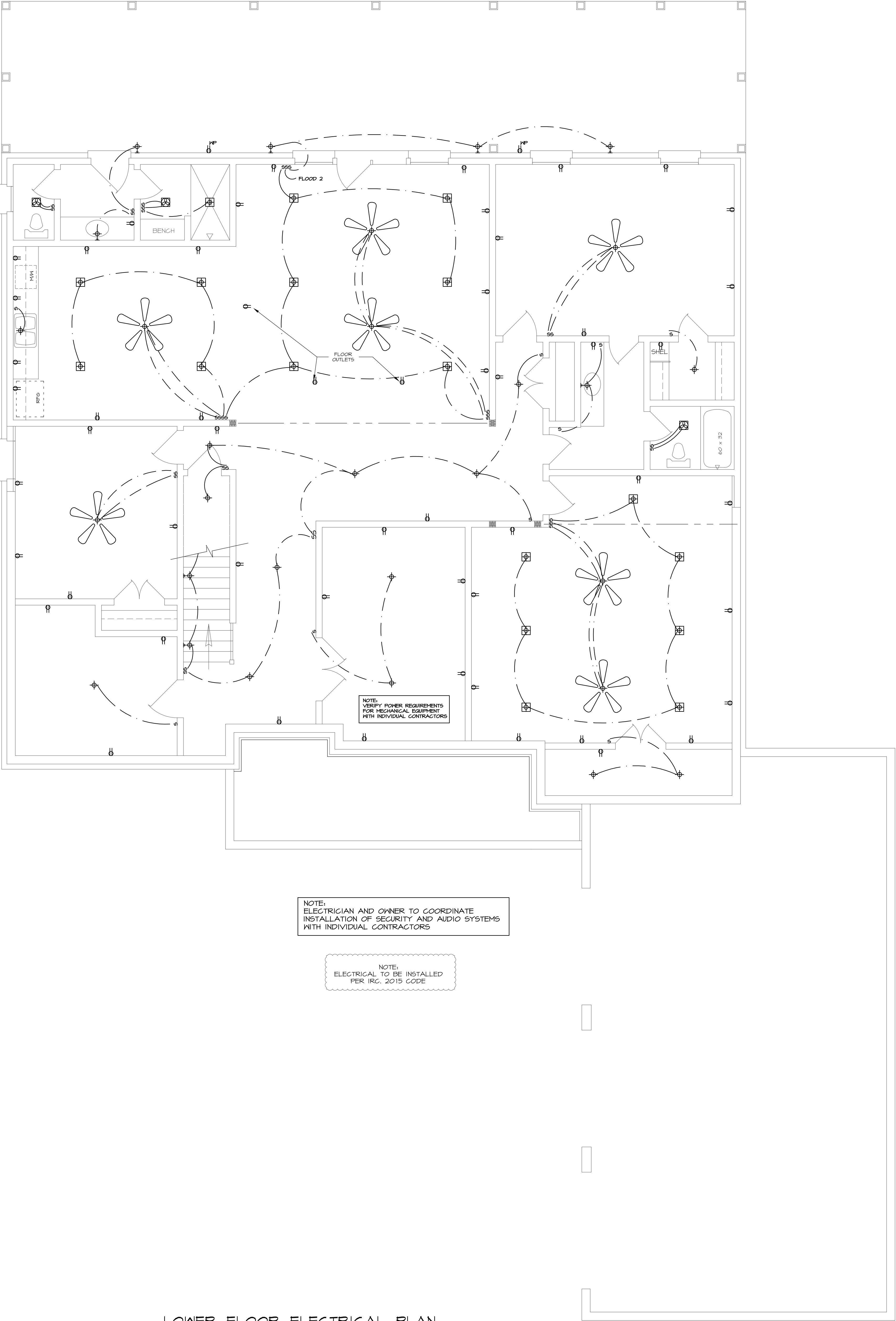
LOWER FLOOR ELECTRICAL PLAN
