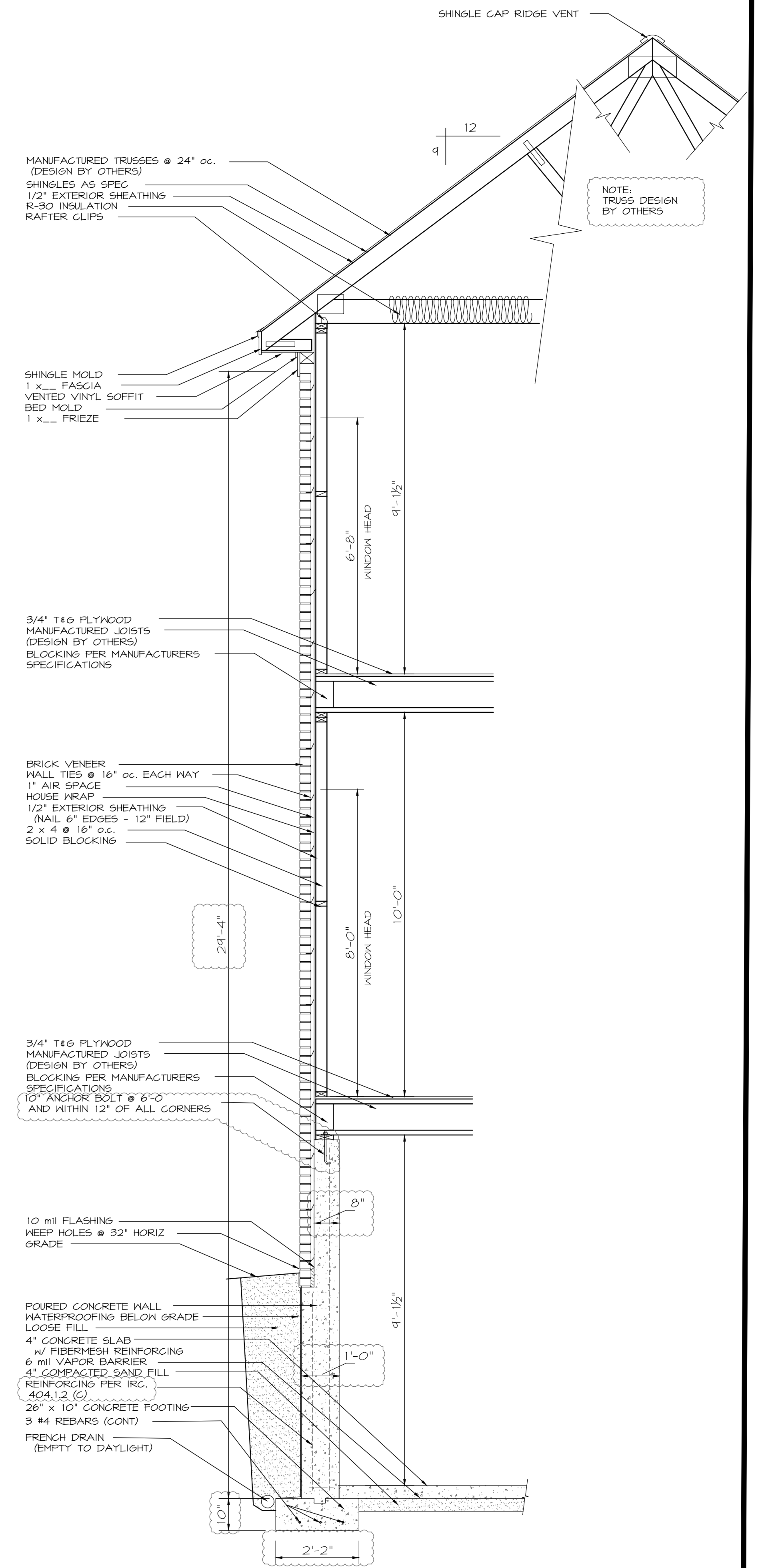
TYPICAL WALL SECTION
