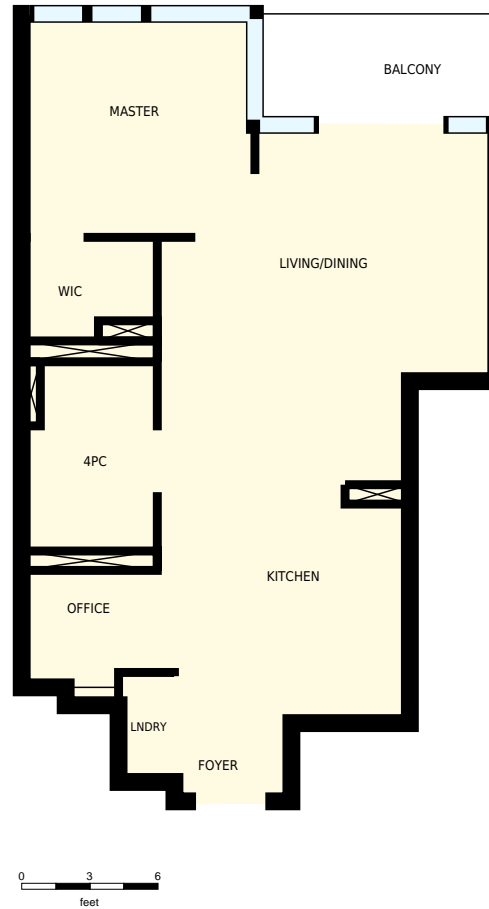
Main floor Exterior Area 640 sq. ft
