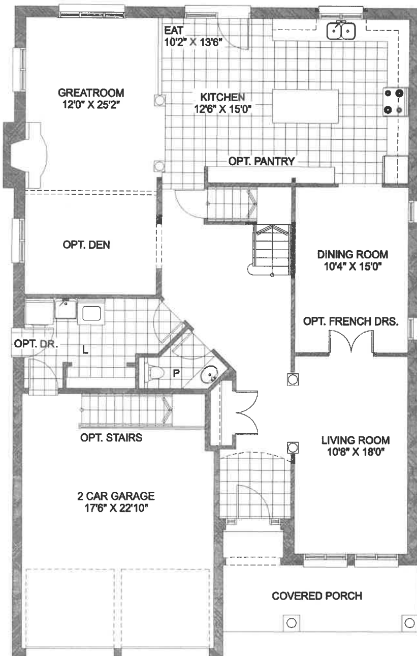
GROUND FLOOR
