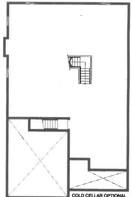
BASEMENT PLAN (Not to Scale)
