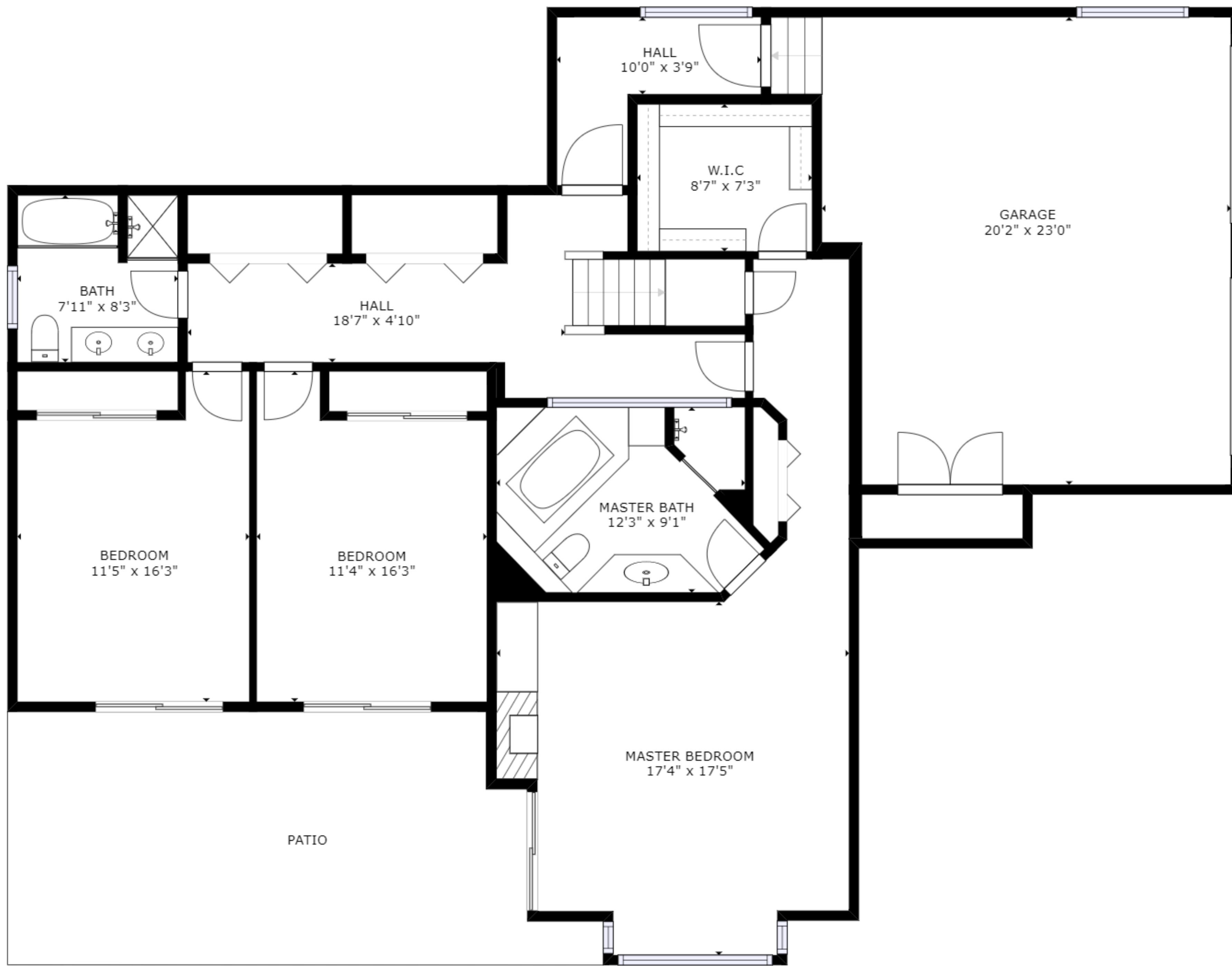
FLOOR 1
