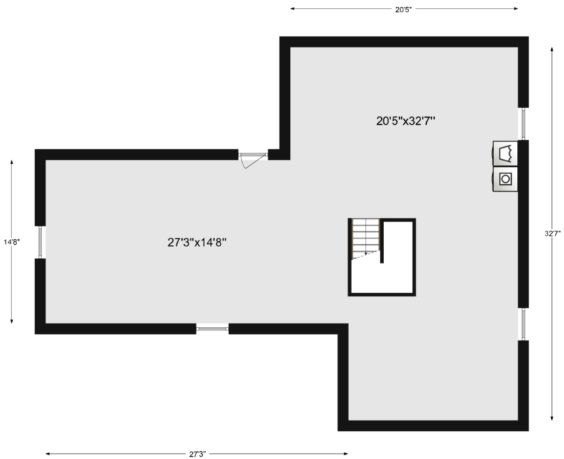
Basement
