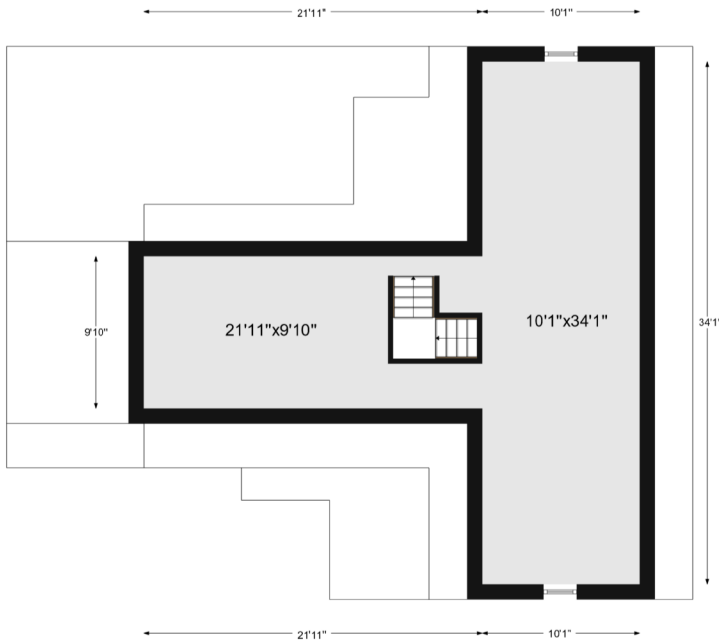
Attic
