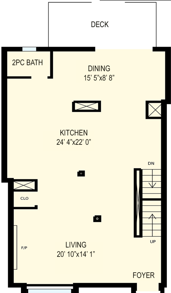
Main Floor Exterior Area 957 sq. ft.
