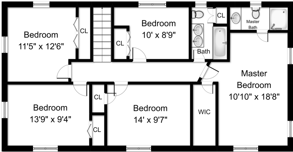
Second Level
