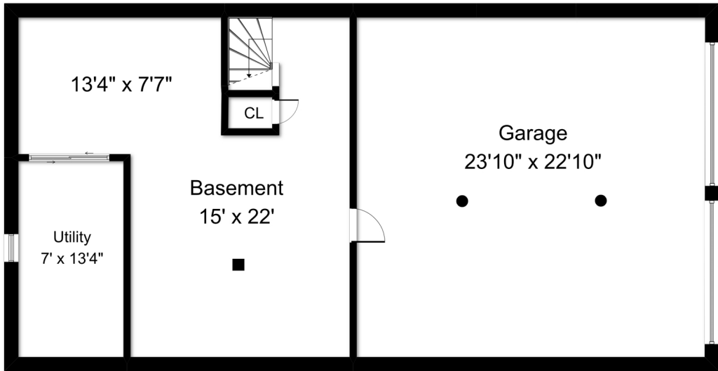
Lower Level
