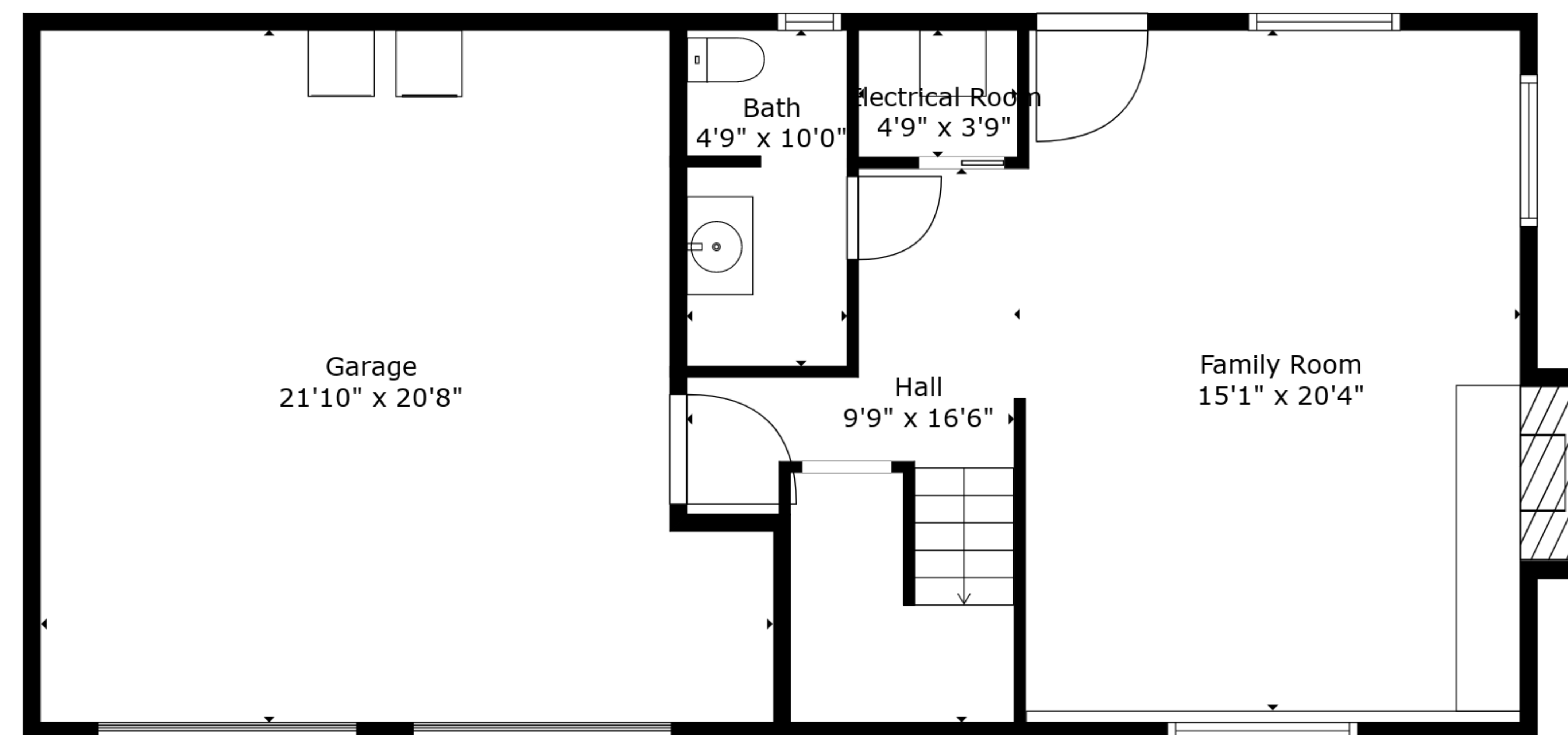
Floor 2
