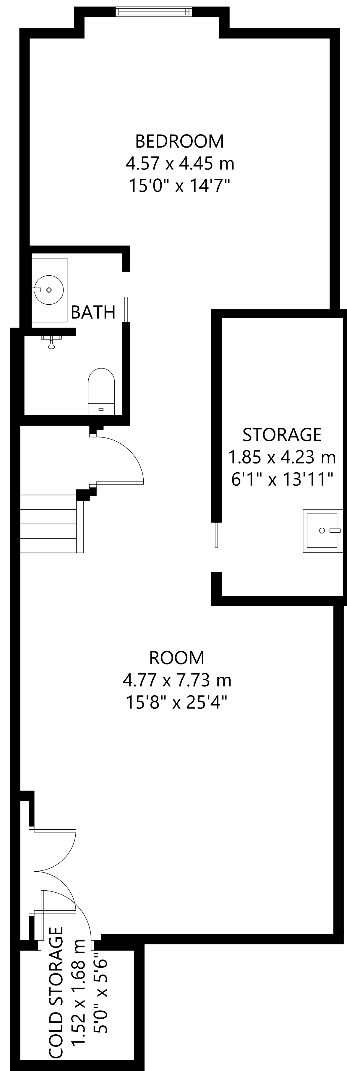
FLOOR 1
