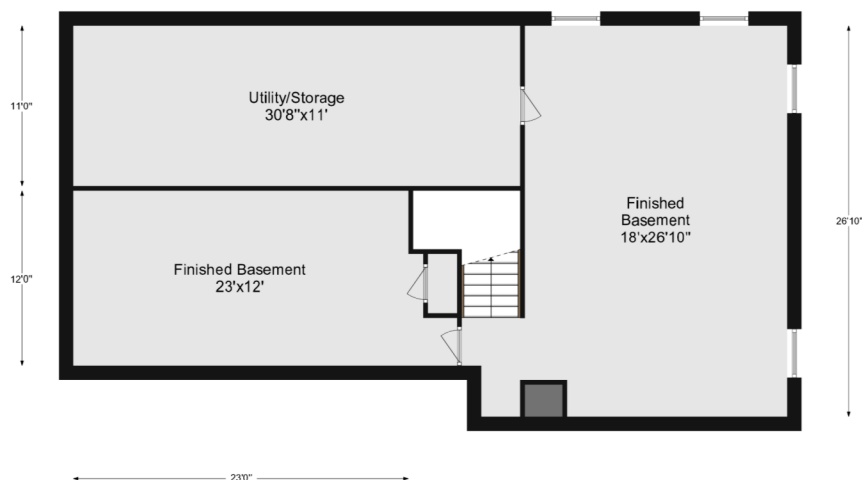
Basement Floor plans are intended to give a general indication of the layout. The information is considered reliable not guaranteed as accurate or complete.
