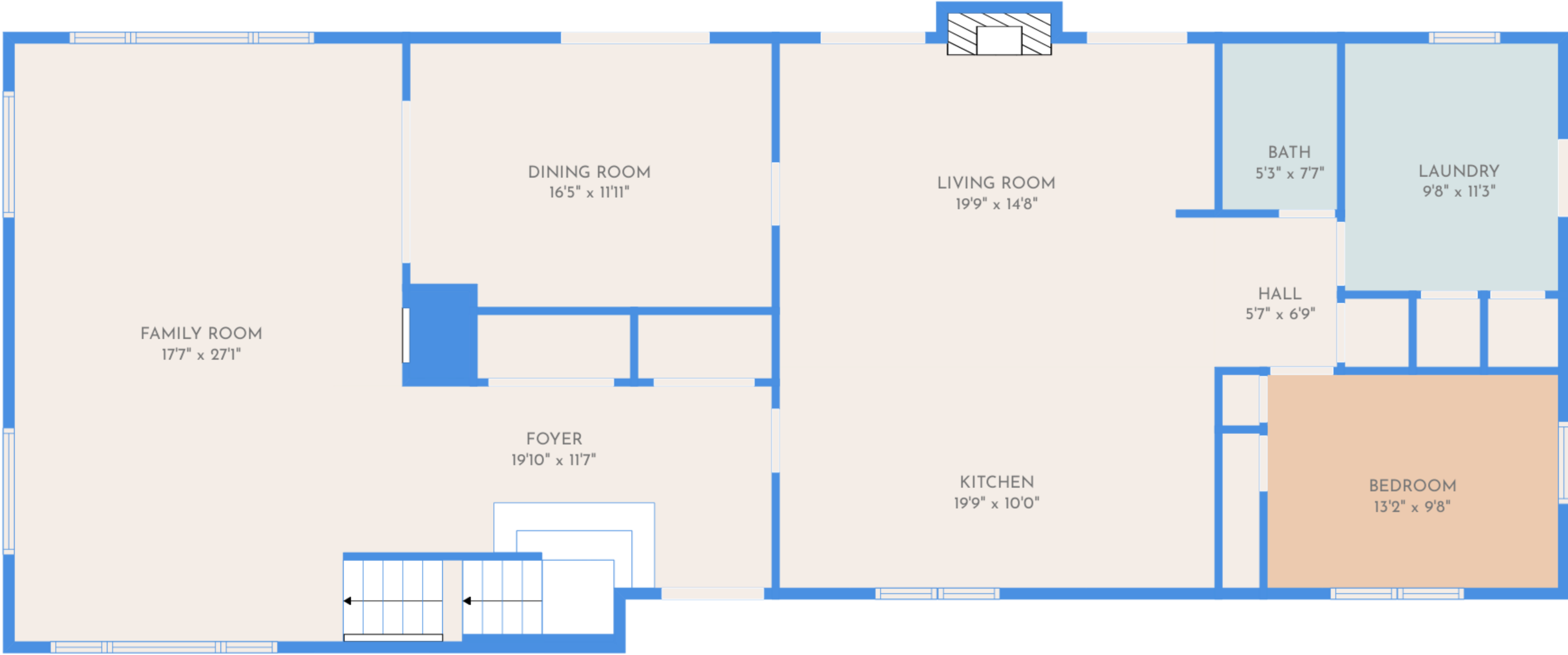
FLOOR 2
