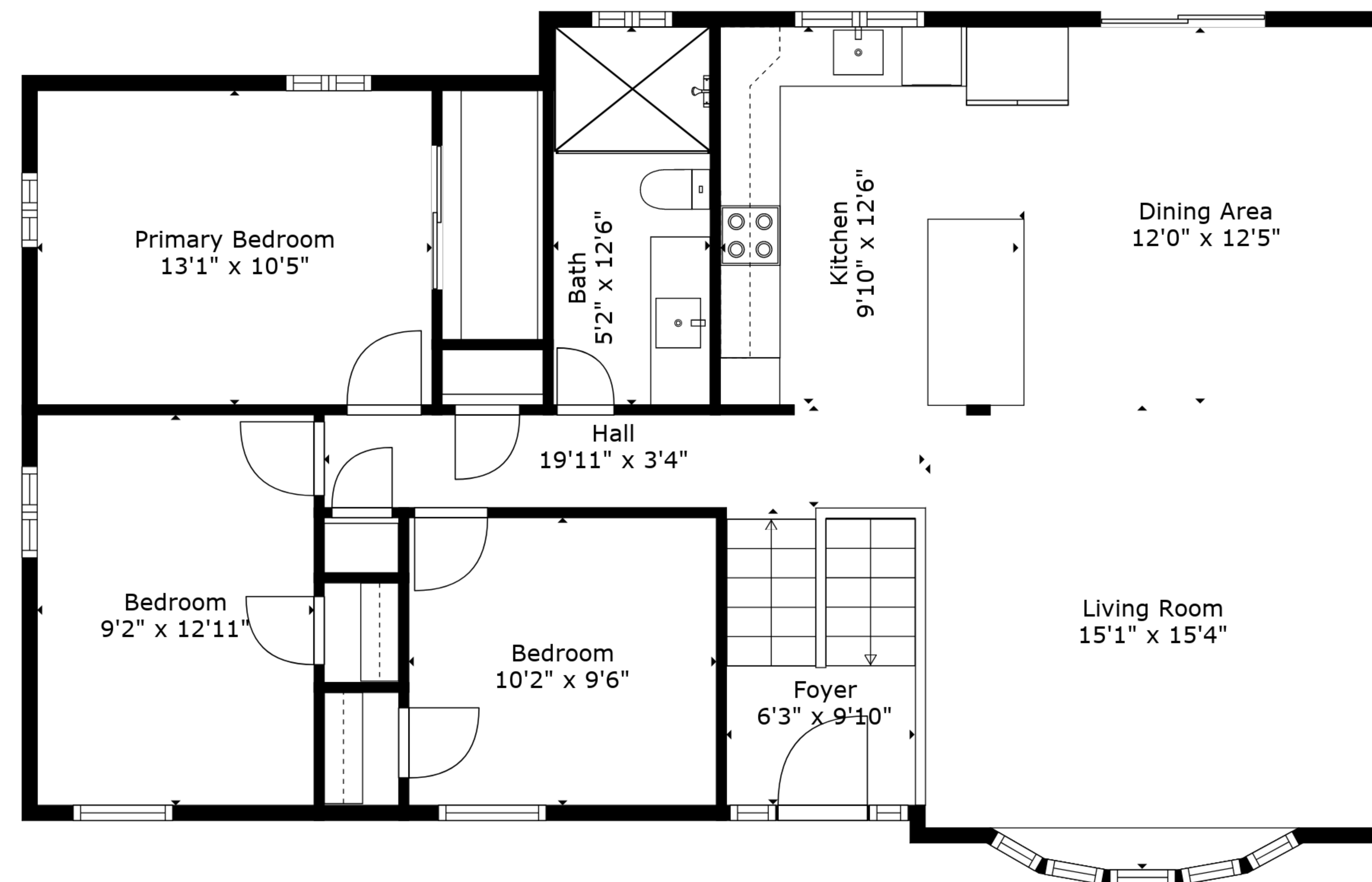
Floor 2
