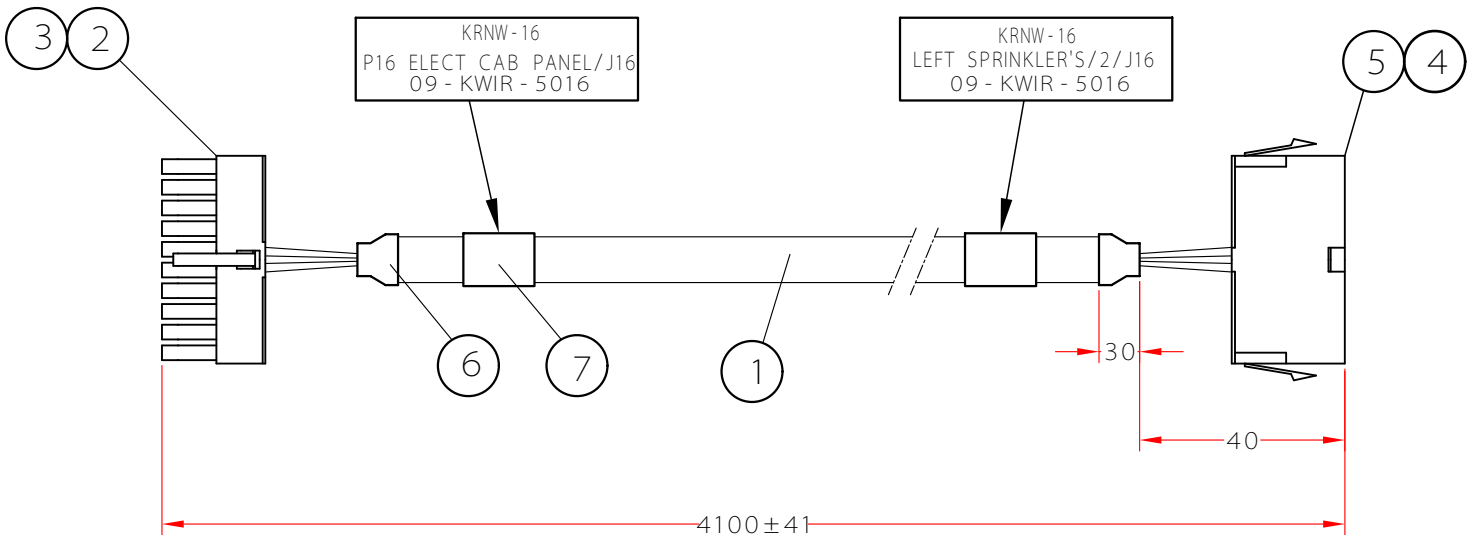
P16 ELECT CAB PANEL/J16
