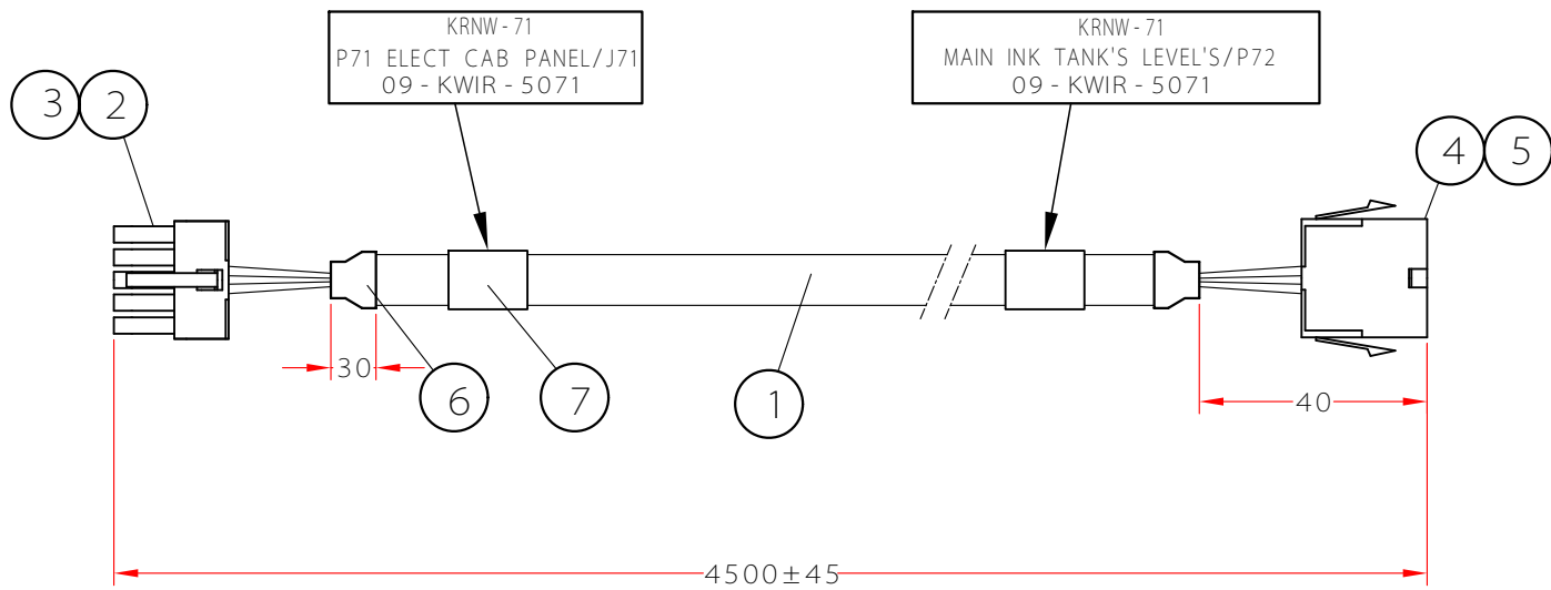
P71 ELECT CAB PANEL/J71
