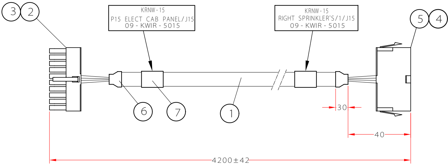
P15 ELECT CAB PANEL/J15
