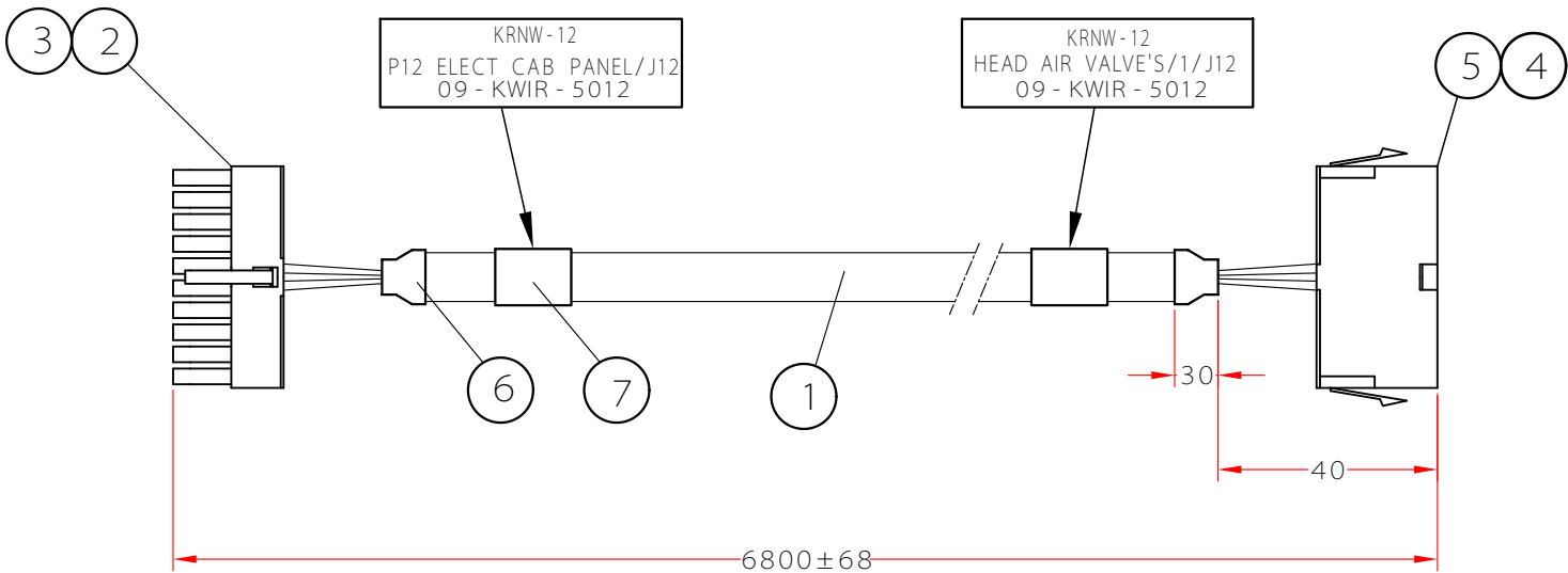
P12 ELECT CAB PANEL/J12
