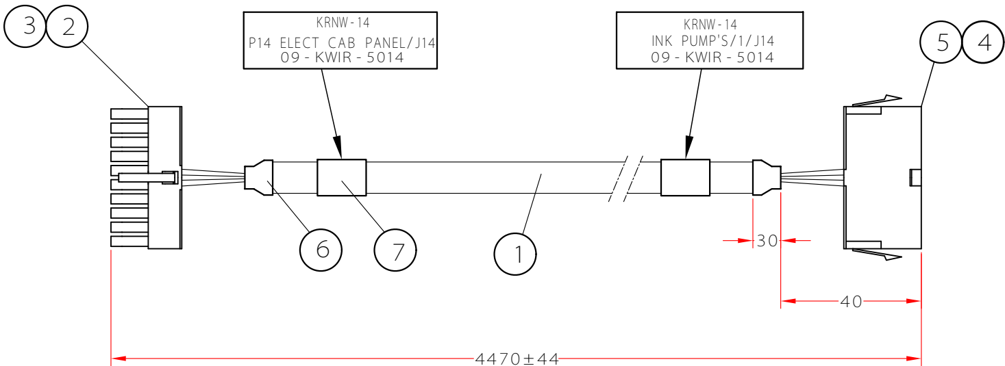
P14 ELECT CAB PANEL/J14
