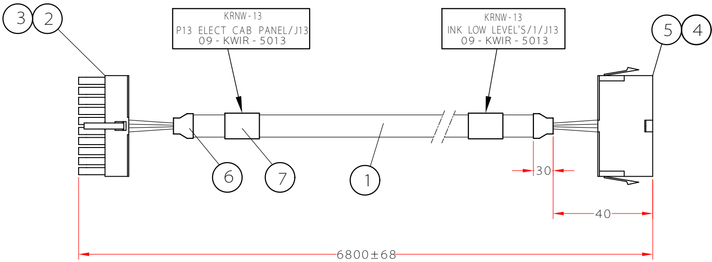
P13 ELECT CAB PANEL/J13
