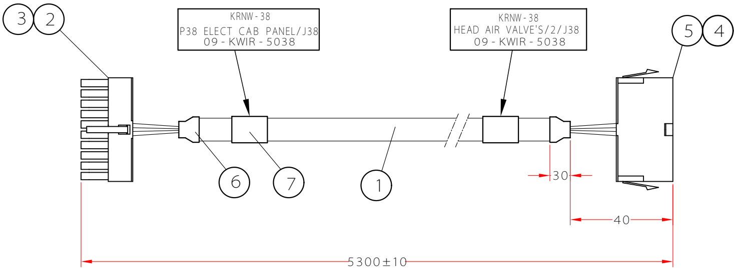
P38 ELECT CAB PANEL/J38
