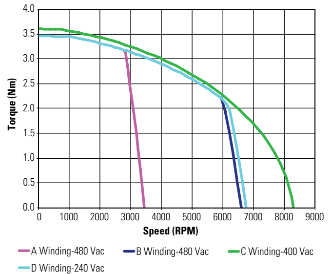
KBM(S)-17X02 Continuous Torque
