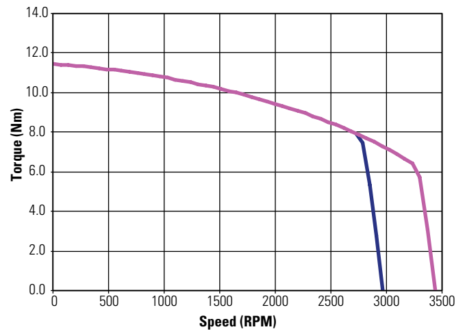
KBM(S)-43X02 Continuous Torque
