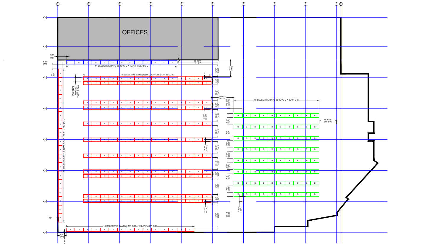
RACK PLAN VIEW
