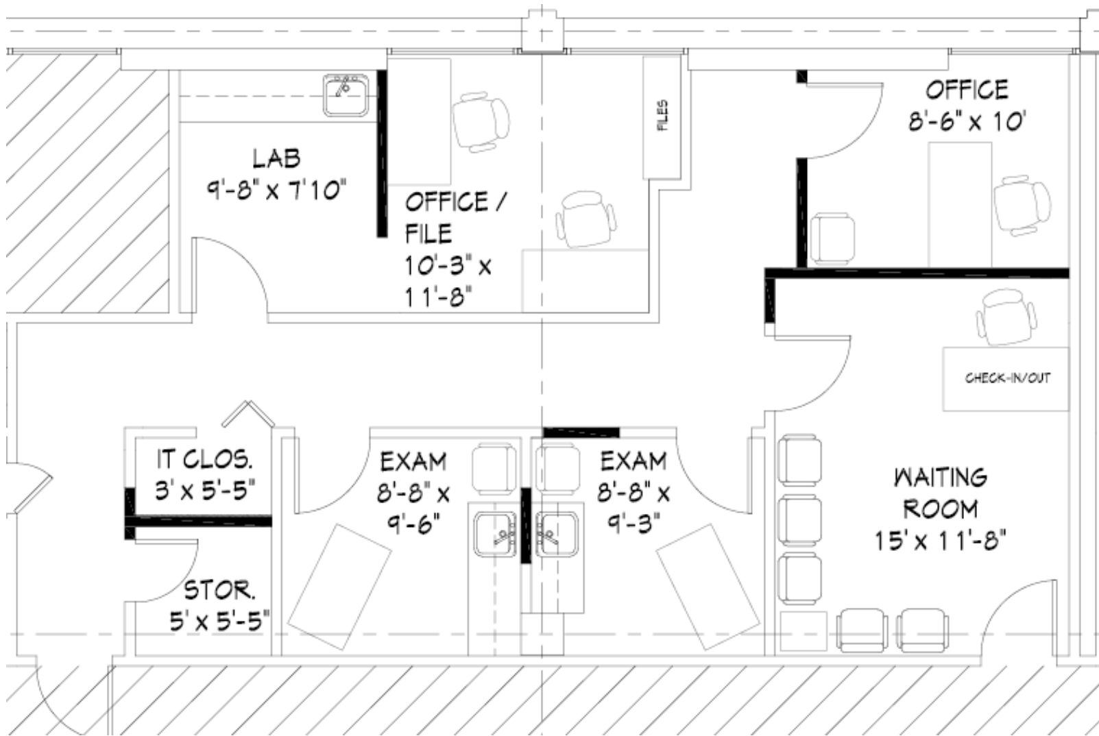
BUILDING PLAN
