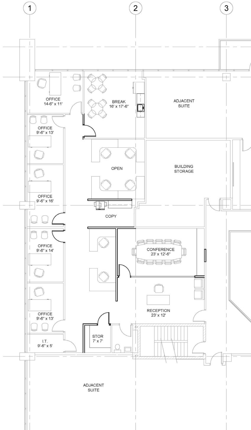
SUITE 255 2,752 SF SCALE 1/8" = 1'-0" 09.24.2020
