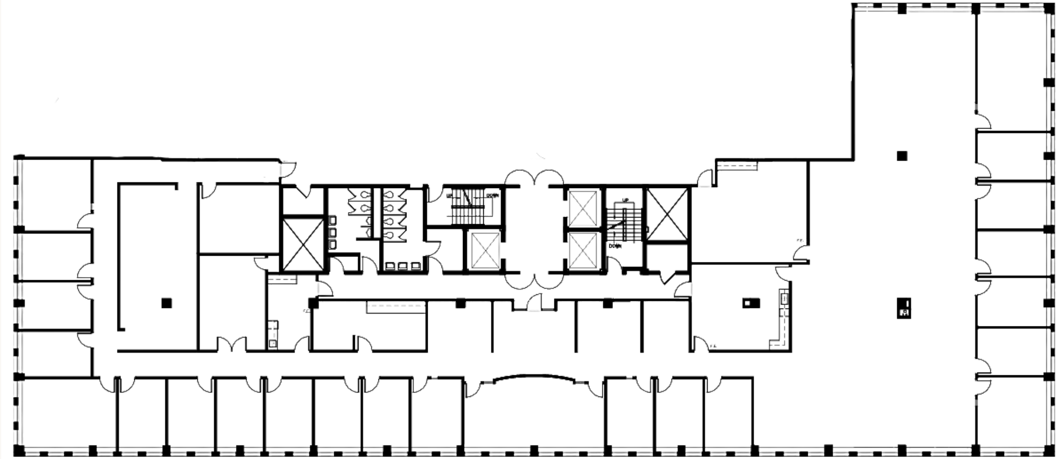
BUILDING PLAN
