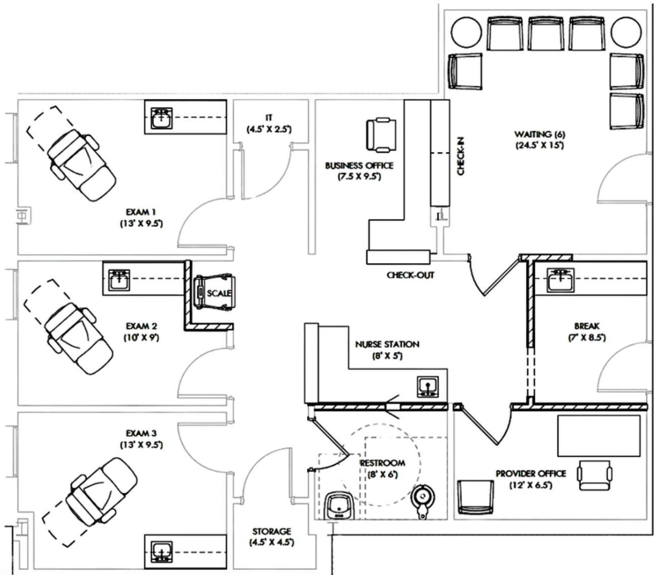
BUILDING PLAN
