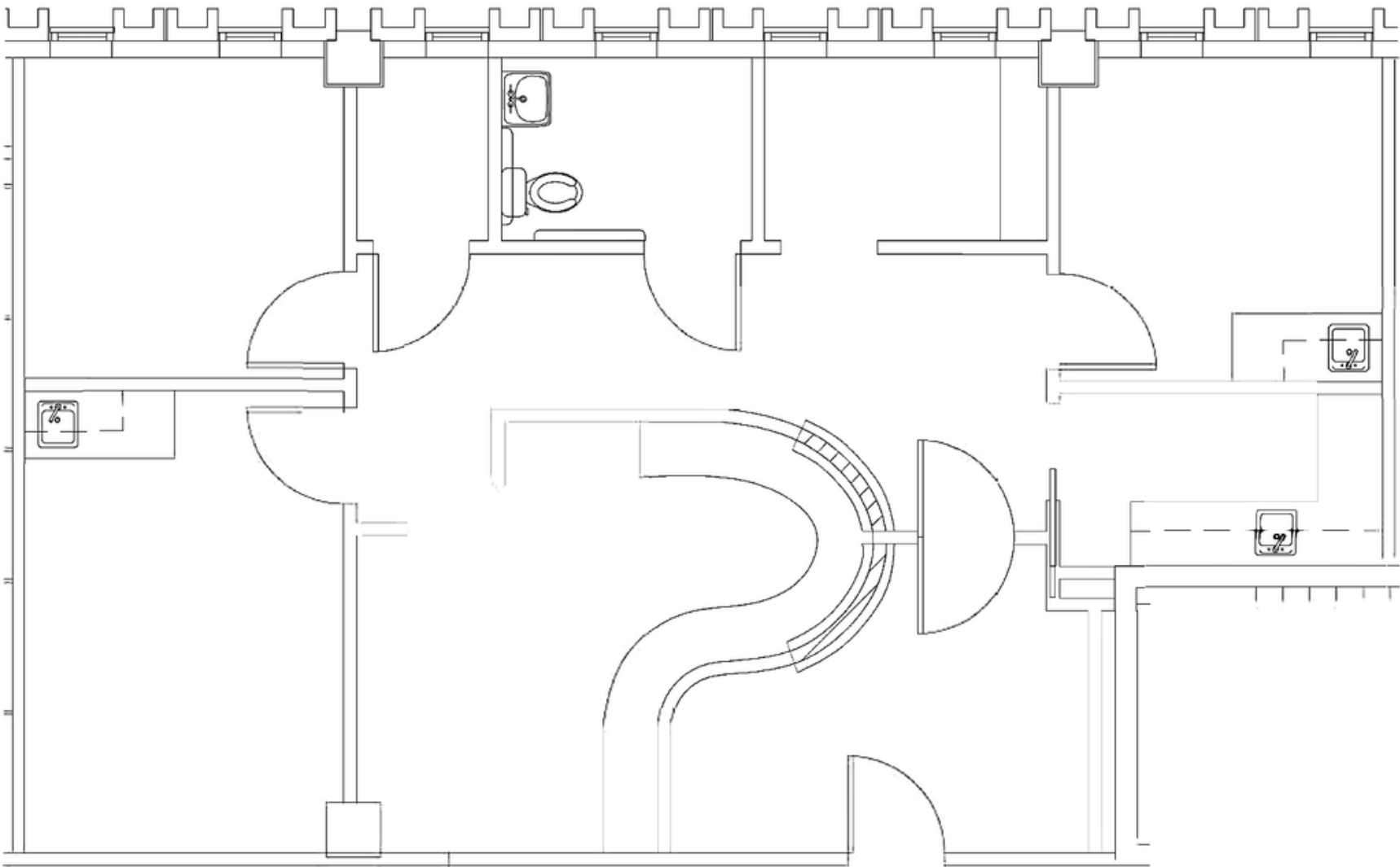
BUILDING PLAN
